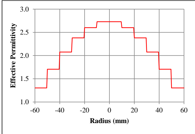
Fig. 2 Effective permittivity values for 3D-printed lens as a function of radius position
