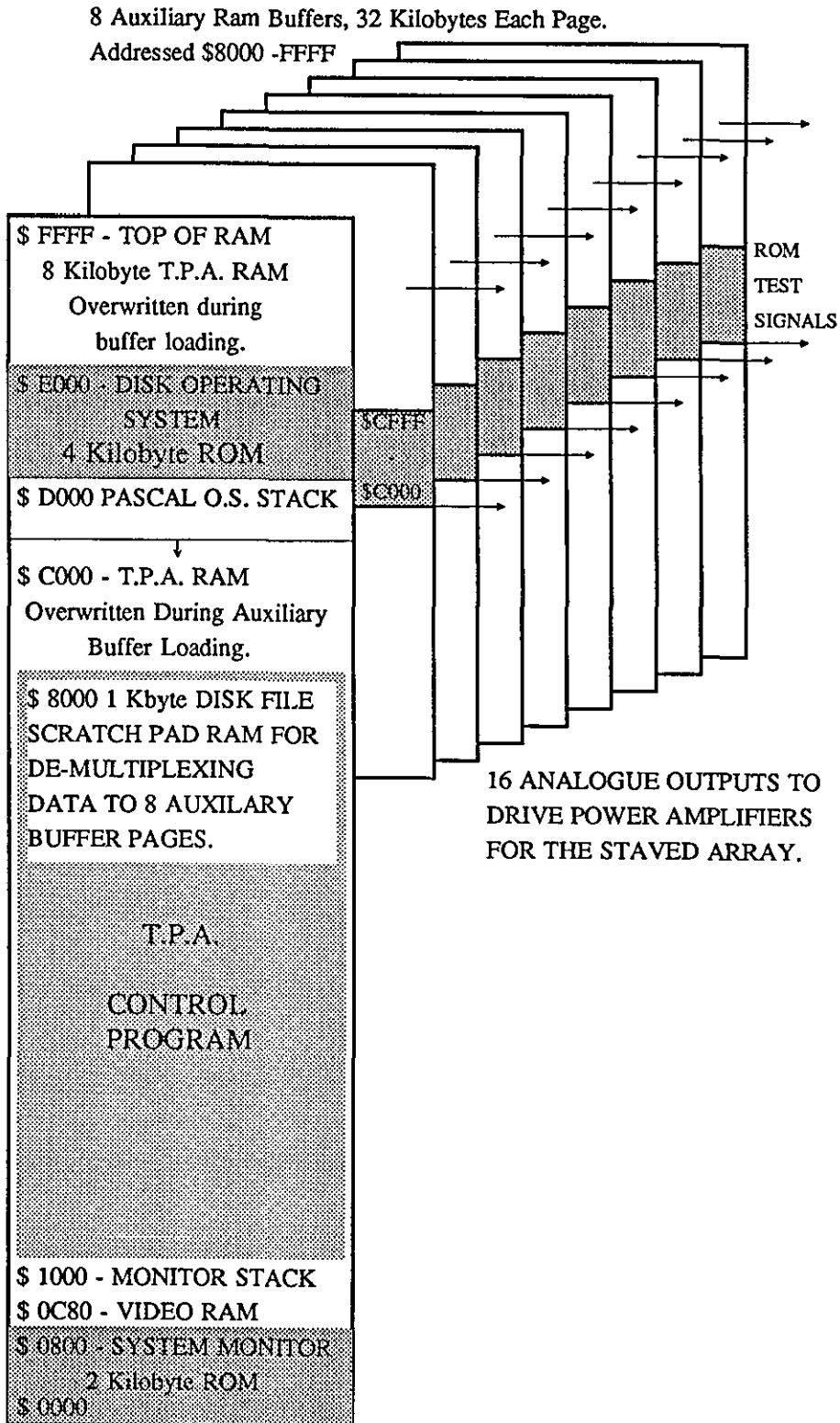
Fig.2.0/5 Block Diagram of the Auxiliary Memory Buffers and the Host Microcomputer Memory Map.
