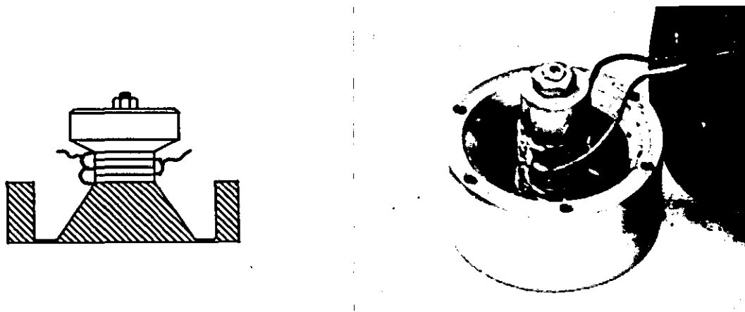
Fig.3.6/1 I.O.S. Transducer - Titanium element construction.
