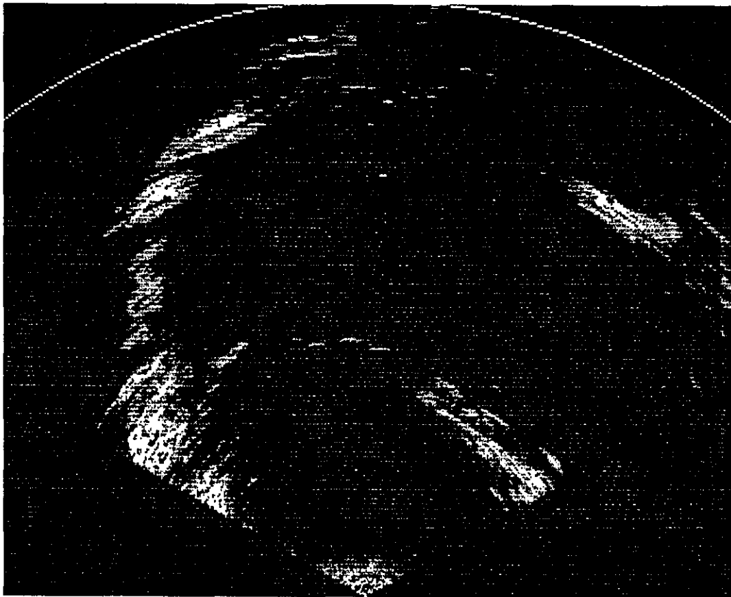
Fig. 3.8/8. Foremark Reservoir Lake Bed. - 800 metre sector, 120 degree mechanical scan, Array tilt is zero.
