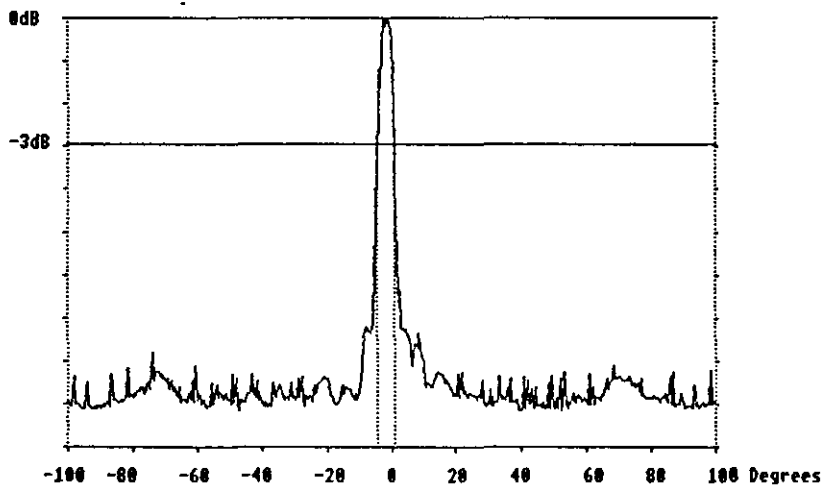
Fig.6.0/2. Mk.1. Array Beam Plot, 200 degree scan.
