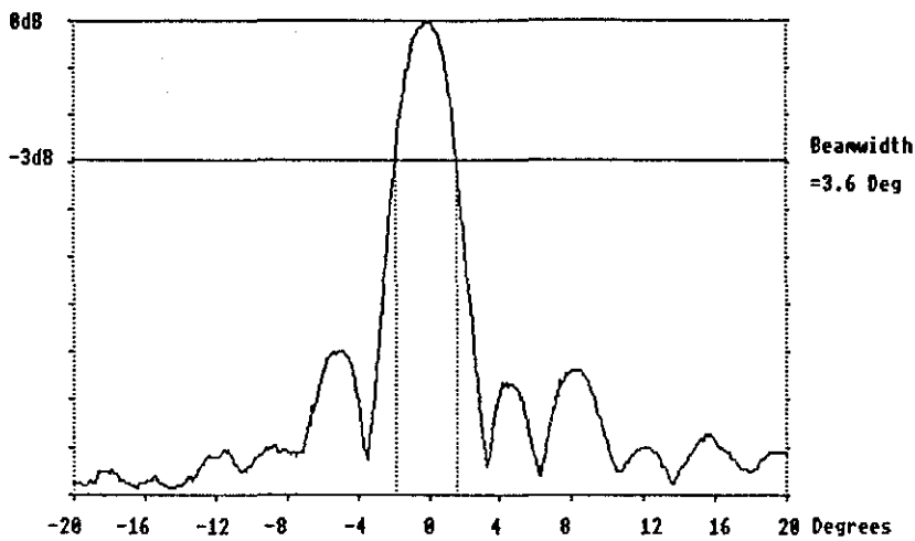
Fig.6.0/3 Mk.1. Array Beam plot, 39 kHz, 40 degree sector.
