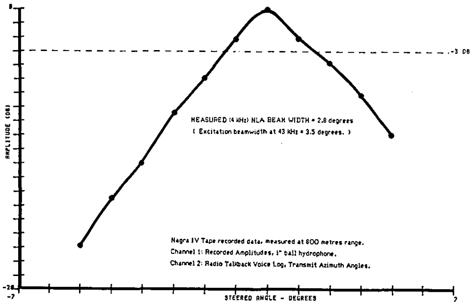
Fig.6.4/2 Foremark experimental determination of the 4 kHz Non-linear beam width.
