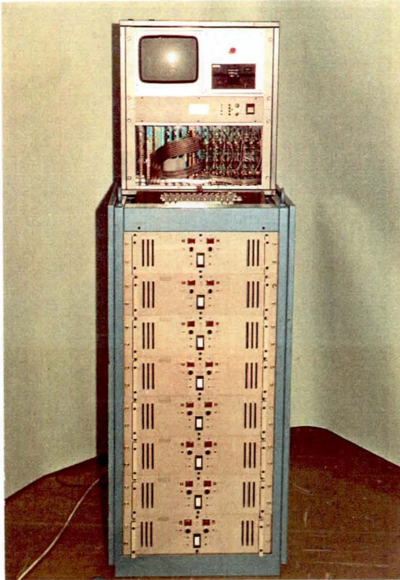
Fig.3.4/2 The complete Mk.2. Transmitter Assembly.
