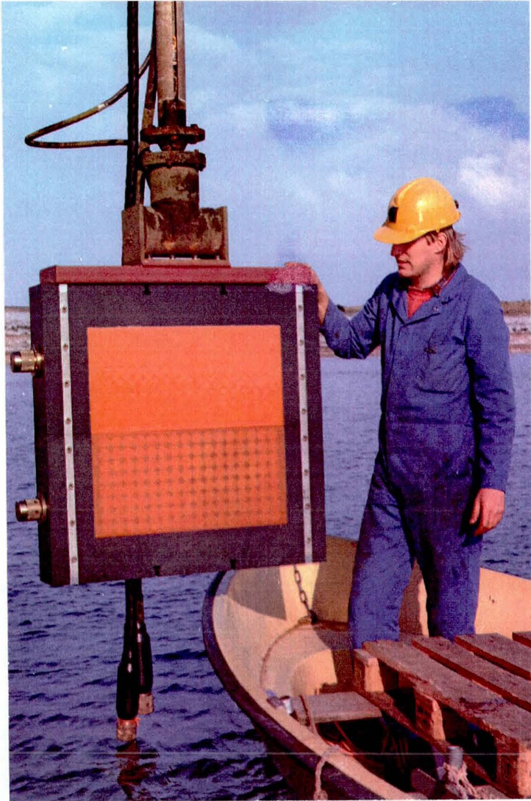
Fig.3.7/1 The Mk.2. Dual Array being deployed at Foremark Reservoir. Each half comprises 16 staves of 8 elements, i.e 16 x 16 in total.
