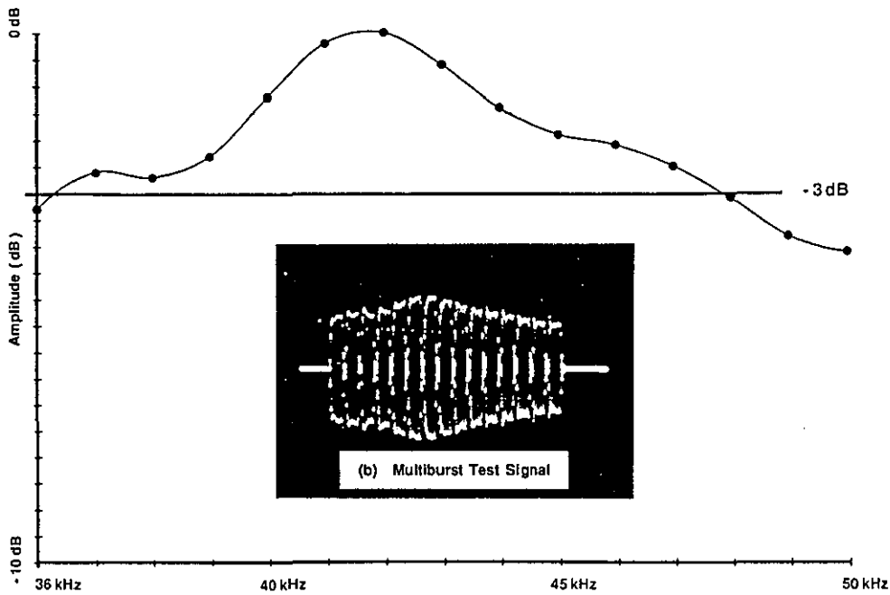
Fig.3.4/1 Frequency response of the complete Mk.2 high power system including the power amplifiers and transducer.
