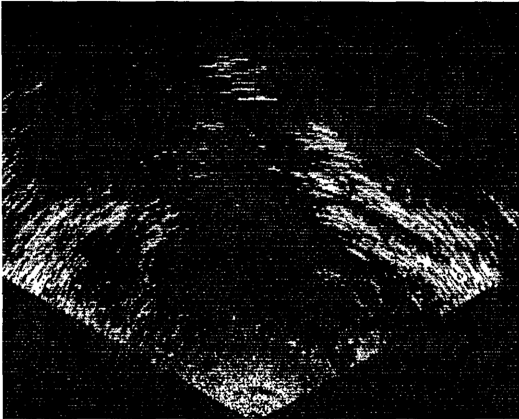
Fig.3.8/7 Foremark Reservoir Lake Bed. - 400 metre sector, 120 degree mechanical scan at 43 kHz, Array tilted down 6 degrees.
