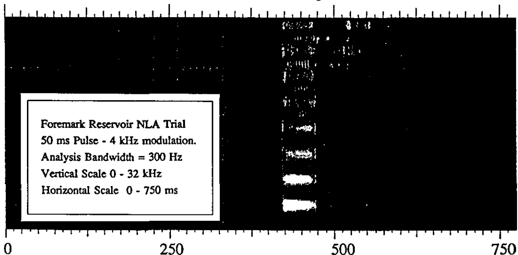
Fig.6.4/1. N.L.A. transmission spectrum. Analysed from data recorded at 800 metres down range.
