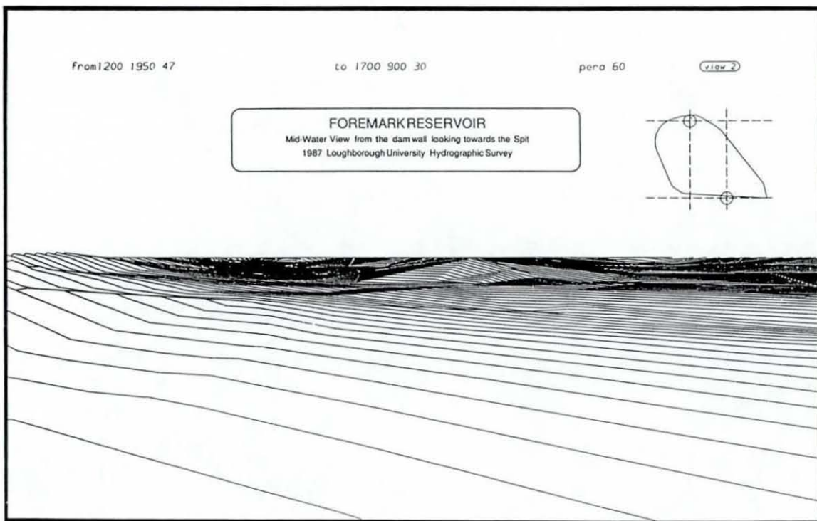
Fig.5.3/3 Underwater Terrain Model of Foremark reservoir, computed from a limited echosounder survey.
