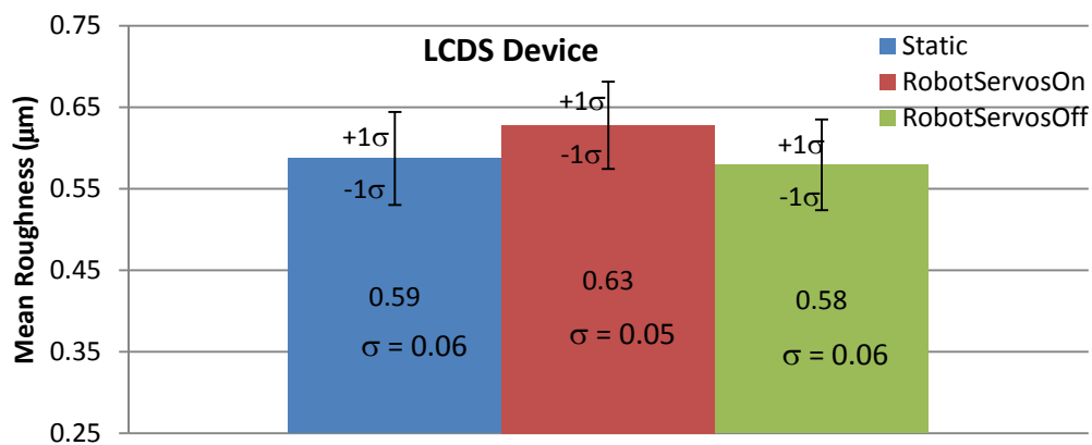
Figure 10: Comparative plots for hole Roughness (Ra)
