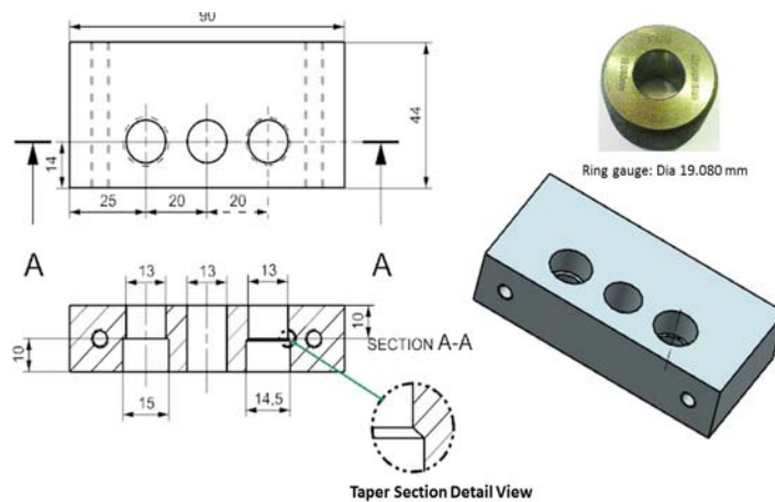
Figure 3: The test part with straight hole, stepped hole and tapered hole
