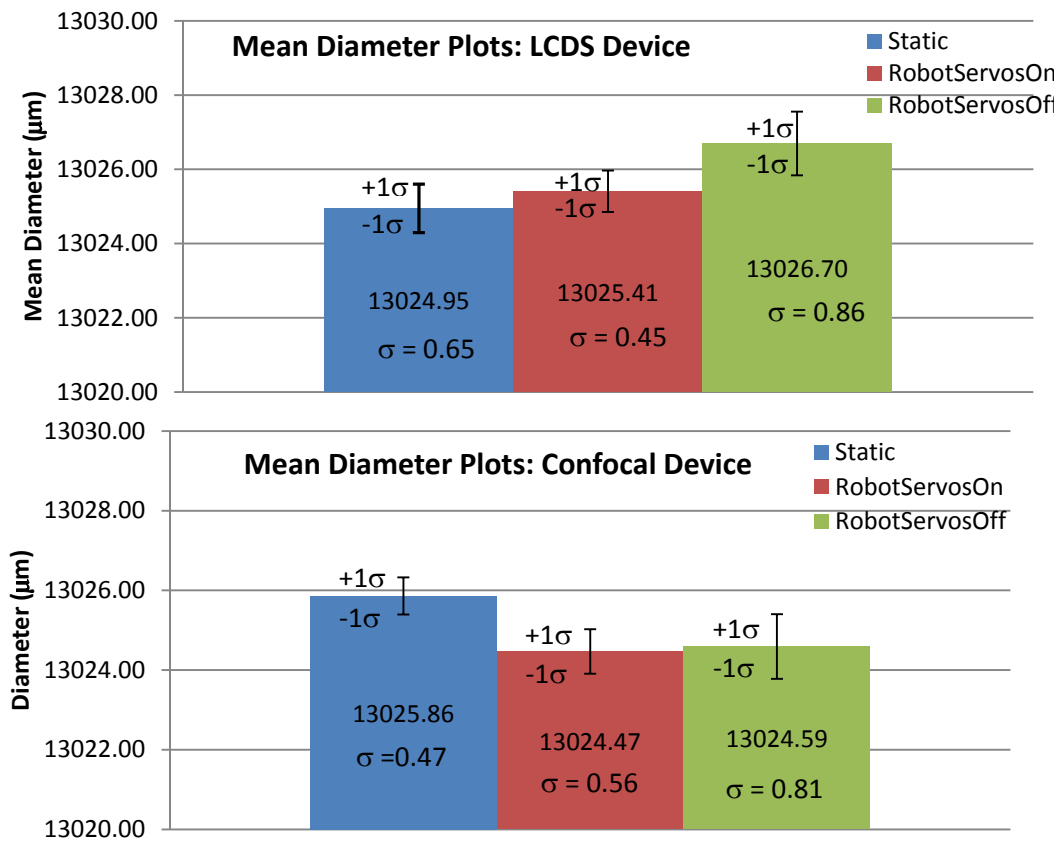
Figure 8: Comparative plots of the mean hole Diameter
