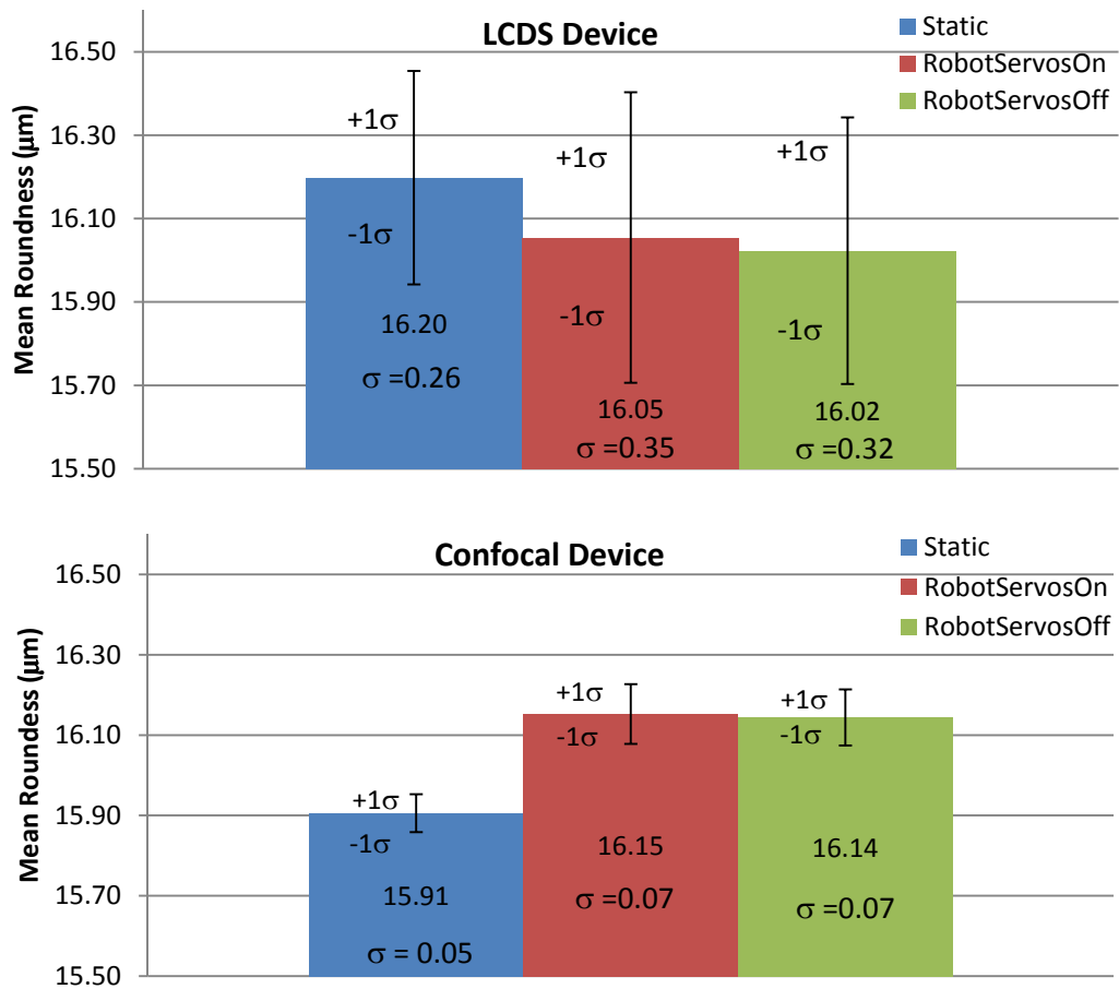
Figure 9: Comparative plots for the mean hole Roundness
