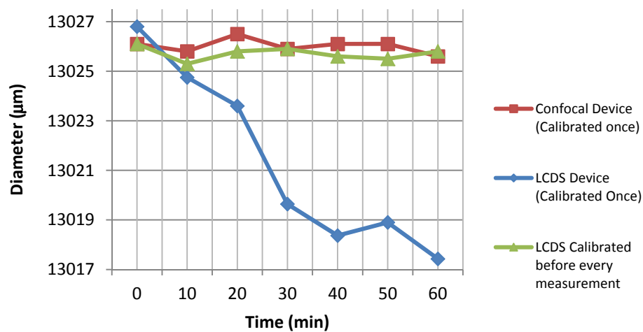
Figure 7: Drift in measurement of confocal and LCDS devices
