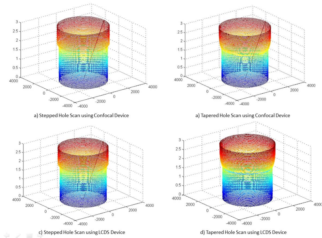
Figure 11: 3D plot of the section containing taper and the section containing step using both the LCDS device and Confocal Device
