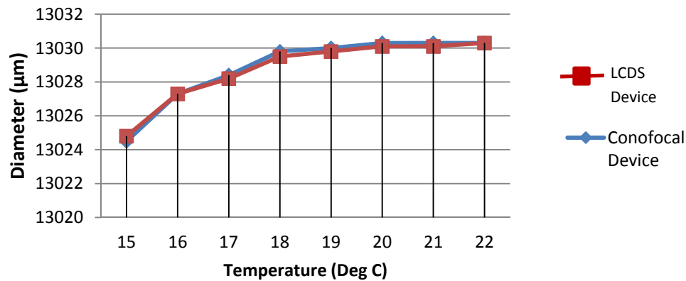
Figure 6: Effect of thermal variations on diameter measurements
