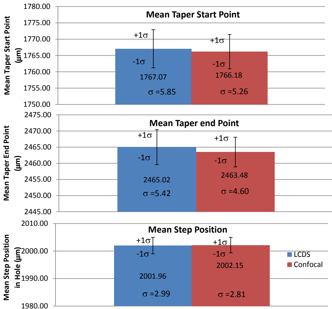
Figure 12: Plots for taper start point, taper end point and hole’s step position from the two devices
