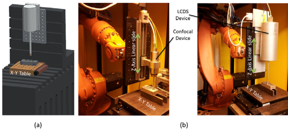
Figure 4: Experiment Setup (a) static platform (b) robotic platforms
