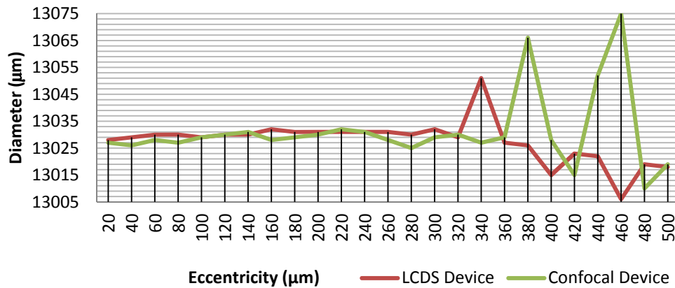
Figure 5: Stability of readings with varying eccentricity
