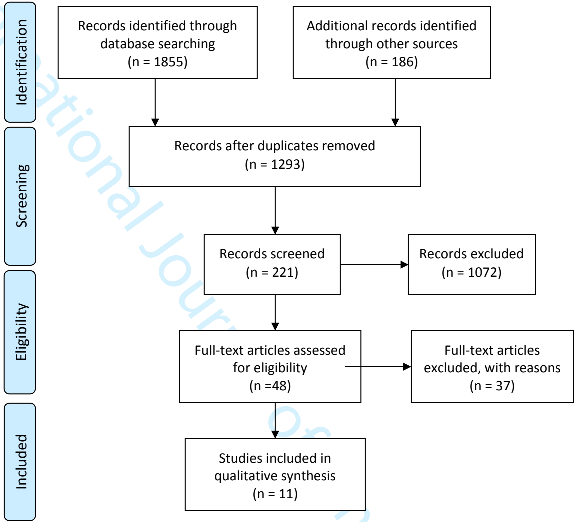
Figure 4. PRISMA diagram
