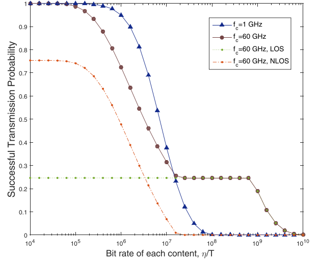
Fig. 5. Successful transmission probability, \lambda_{\mu,mm} = 400/\text{km}^2 , b_j = 1 .
