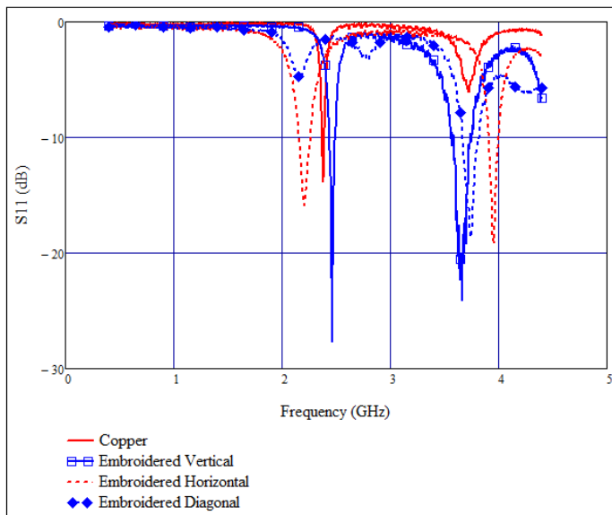
Figure 5. S_{11} Values for the four antennas in Figure 4.
