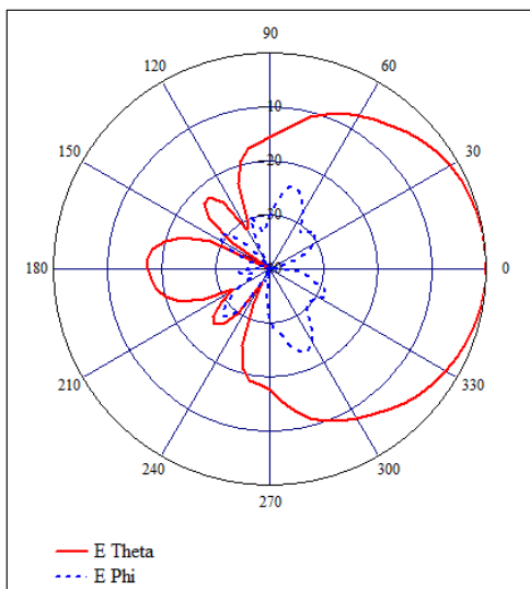
Figure 4.d. Representative Antenna Cut for Etched Copper Patch Antenna at 2.3825 GHz. Patch antenna faces to the right with the longer side parallel to the plane containing the cut.
