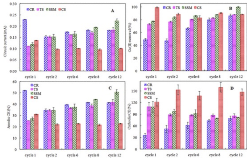
Fig. 2 Circuit current (A), Cu(II) removal (B), anodic CEs (C) and cathodic CEs (D) in MFCs with various material cathodes as a function of time.
