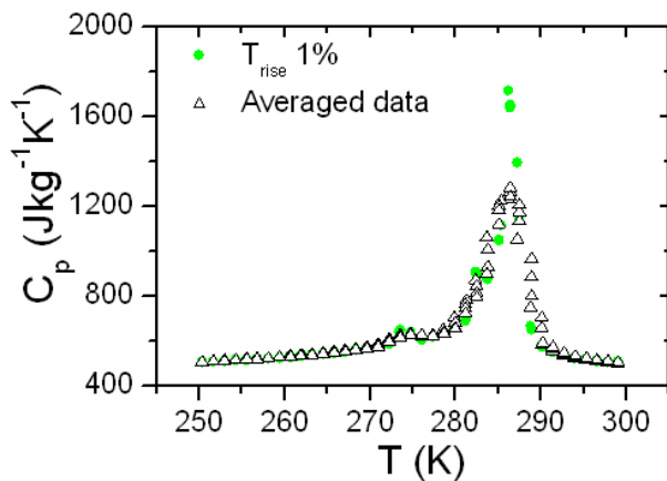
Fig. 6 – Impact of experimental parameters on PPMS measurements (colour online). Graph shows the result of averaging heat capacity over a large temperature window ( \sim 2\%T_{\text{bath}} ) where the sharp change in heat capacity now resembles broad behaviour observed in the pellet.
