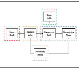
Figure 5: Architecture of CLM of smart transmitter
