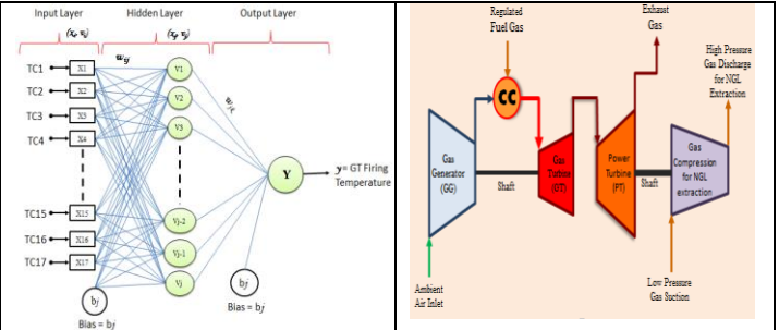
Fig 8: simplified model of a feedforward neural network (FFNN) Fig 9: Abstraction of gas processing system
