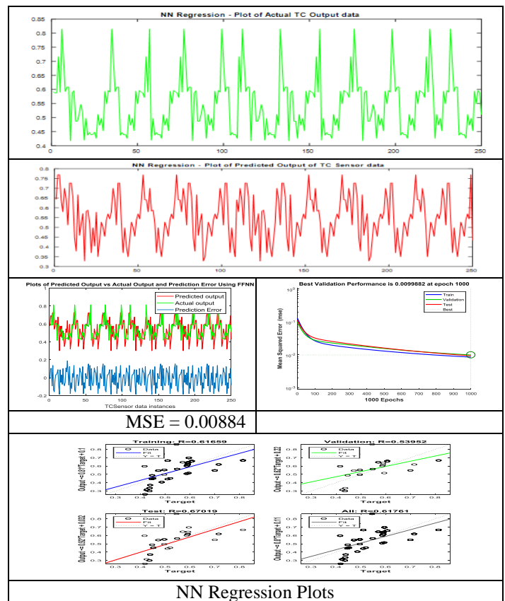
Fig 10: Result of MSDF of GT Firing temperature sensors data using FFNN
