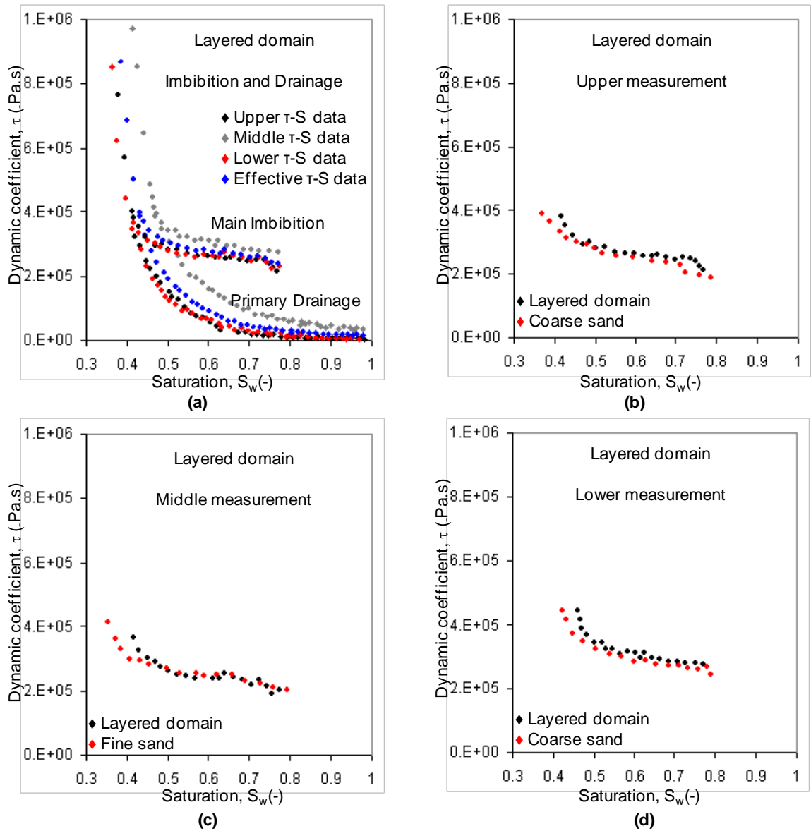
Figure 12. Hysteresis in primary drainage and main imbibition \tau - S_w curves in heterogeneous domain: (a) primary drainage and main imbibition \tau - S_w curves in heterogeneous domain, (b) main imbibition \tau - S_w curves in the upper measurement points (coarse sand) in heterogeneous and homogeneous coarse sand domains, (c) main imbibition \tau - S_w curves in the middle measurement points (fine sand) in heterogeneous and homogeneous fine sand domains (d) main imbibition \tau - S_w curves in the lower measurement points (coarse sand) in heterogeneous and homogeneous coarse sand domains
