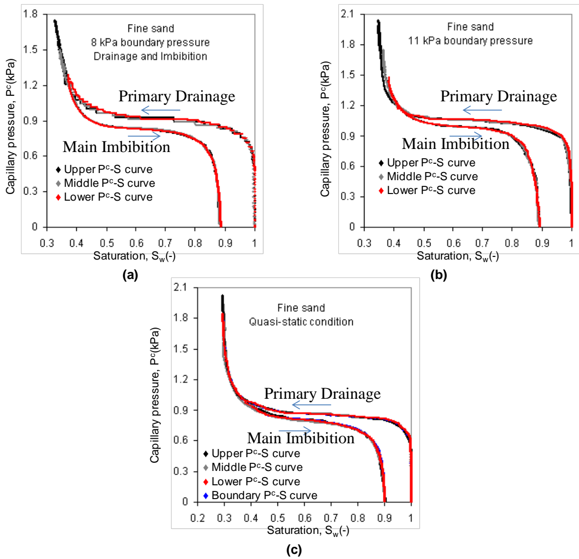
Figure 9 (a-c): Primary drainage and main imbibition P^c - S curves showing hysteresis in fine sand (a) hysteresis in dynamic drainage and imbibition P^c - S curves for 8 kPa pressure; (b) hysteresis in dynamic drainage and imbibition P^c - S curves for 11 kPa pressure; (c) hysteresis in quasi-static drainage and imbibition P^c - S curves
