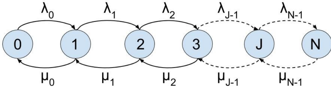
Figure 5 The (generic) Transition Diagram for the CTMC of the transport model
