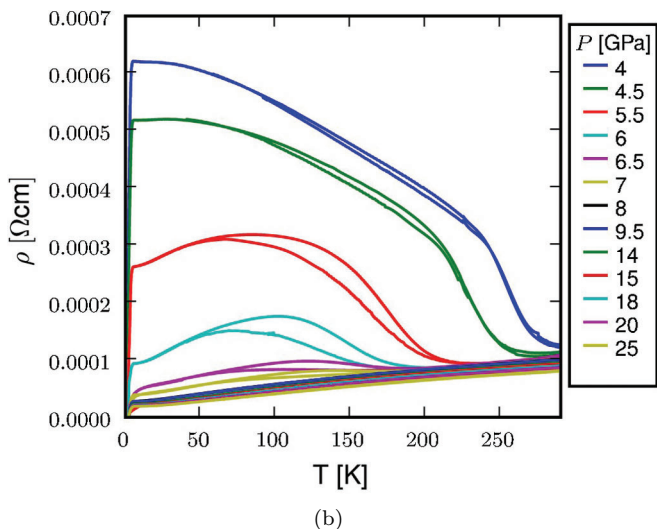
Figure 2: Resistivity in the pressure range of 0–25 GPa and temperature range of 1.3–300 K. Figure a shows that the temperature dependence of the resistivity is largely non-metallic over the entire temperature range for pressures of 0–4 GPa; the low temperature upturn in the resistivity that relates to the variable-range-hopping conduction in the Mott phase 11,12 disappears above 0.6 GPa; first traces of the superconductivity are observed at an approximate pressure of 2.5 GPa, with a T_{SC} of 1.5 K; metallic-like behaviour develops for low temperatures at pressures of 4–8 GPa; fully metallic behaviour is present at pressures greater than 8 GPa. Figure b clearly demonstrates that the superconductivity first develops with pressure within the non-metallic phase.
