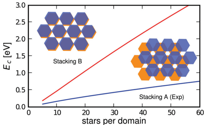
Figure 4: The results for the Coulomb energy calculation for two different domain stacking as a function of domain size. The lower line (blue), corresponds to an axial arrangement of domains (hexagonal) and interdomain spaces (triangular) between adjacent layers (stacking A), as deduced from experiment; 28 the upper line (red) shows, for comparison, the Coulomb energy for a hypothetical axial domain stacking between successive layers (stacking B). The green dashed box depicts the values of domain sizes that were experimentally observed in the NCCDW phase at ambient pressure. We note that the Coulomb energies calculated for these values are comparable to the energy of the gap, hinting at a possible Coulomb-controlled phase separation.
