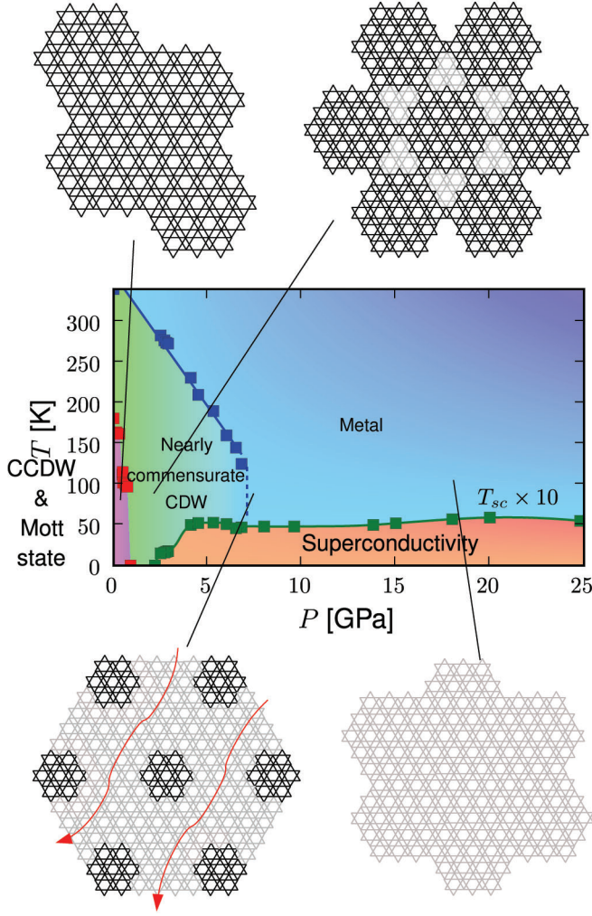
Figure 3: The temperature-pressure phase diagram of 1T-TaS 2 . The Mott localization is suppressed, closely accompanied by the melting of the commensurate CDW phase at a pressure of 0.8 GPa; the lattice structure in the latter phase is composed of interlocking David stars. The nearly commensurate CDW phase extends over the pressure range of 1–7 GPa, and may be visualised as roughly hexagonal domains suspended in an interdomain phase, indicated in grey. The first signatures of superconductivity appear from the nearly commensurate CDW state, and remain roughly at 5 K throughout the entire pressure range of 3–25 GPa. In the pressure range of 8–25 GPa the system is metallic over the investigated temperature range when above the superconducting transition temperature. The drawing above and below the phase diagram indicates the probable deformation patterns in the system at low temperature, as discussed in the text. Darkly shaded parts denote the parts with the static deformation in the form of David stars, while in the light-shaded areas the deformation is considerably reduced or completely suppressed.
