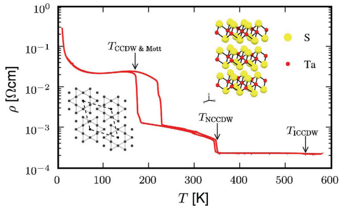
Figure 1: Ambient pressure phases of 1T-TaS 2 . The phases are: a metallic phase at temperatures above 550 K; a charge density wave phase (ICCDW) above 350 K; a nearly commensurate charge density wave phase (NCCDW) above 190 K; a commensurate charge density wave CCDW Mott phase below 190 K; additionally there is a trigonal phase present solely during the warming up cycle between 200–300 K. 9,10,19 Also shown are the Ta atom distortions in the fully commensurate phase (see insert at low temperatures) and the crystal structure of 1T-TaS 2 .
