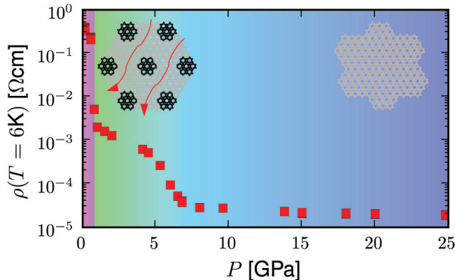
Figure 5: Resistivity taken at a temperature of 6 K as a function of pressure. Sharp decrease in resistivity accompanies the suppression of the Mott-localised phase; linear residual resistivity pressure dependence accompanies the gradual melting of the CDW domains in the nearly commensurate CDW phases; a shoulder-like anomaly in the pressure range 4–7 GPa may be associated with the complete dissociation of the CDW domains with pressure; above 7 GPa the residual resistivity again behaves linearly with pressure. The scattering of electrons on the CCDW islands dominate the resistivity below 7 GPa
