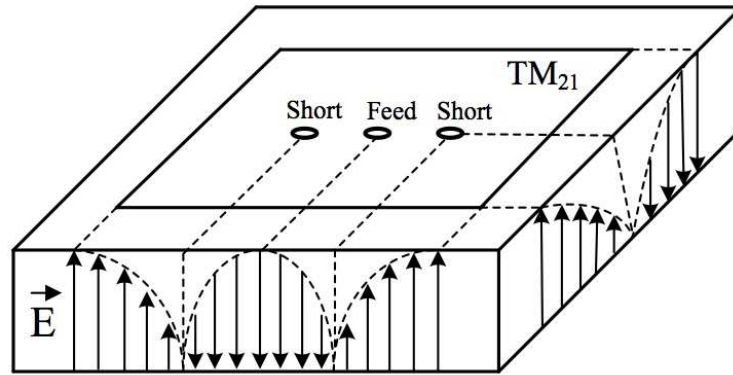
Fig. 3. Theoretical electric field distribution of the TM_{21} mode of HMMPA antenna
