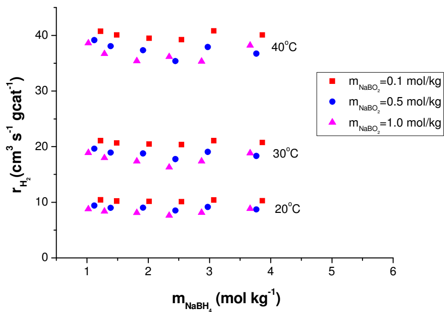
Fig. 6. Hydrogen generation rate versus the molality of \text{NaBH}_4 . The data was obtained by data analysis method introduced in section 2.4 after conducting the experimental programme in Table 2. The catalyst was 0.3 g with an average particle size of 0.049 mm.
