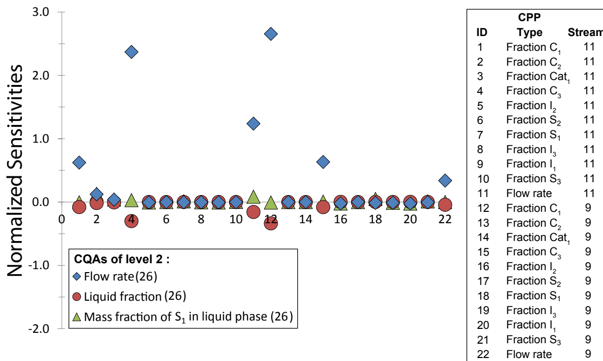
Figure 10: Steady-state values of the normalized sensitivities of the CQAs of Level 2 with respect to the CPPs at Level 3. The stream numbers refer to 1. The fraction of the various compounds in the table with CPPs represents the mass-based fraction of a compound in the liquid phase. The liquid fractions are volume-based liquid fraction of a slurry. The numerical values of the sensitivities are available as Supplementary Material.
