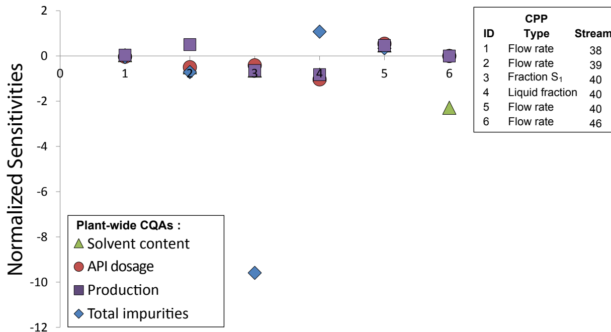
Figure 8: Steady-state values of the normalized sensitivities of the CQAs of the final product with respect to the available manipulated variables for Block 2C of the decomposition (see 5). In the legend, “Fraction S_1 ” refers to the mass-based fraction of solvent S_1 in the liquid phase and “Liquid fraction” refers to the volume-based liquid fraction of the slurry. The CPPs with ID 4, 5, and 6 can be manipulated by changing the setpoints of control loops that are established around Block 2A (see 4). The numerical values of the sensitivities are available as Supplementary Material.
