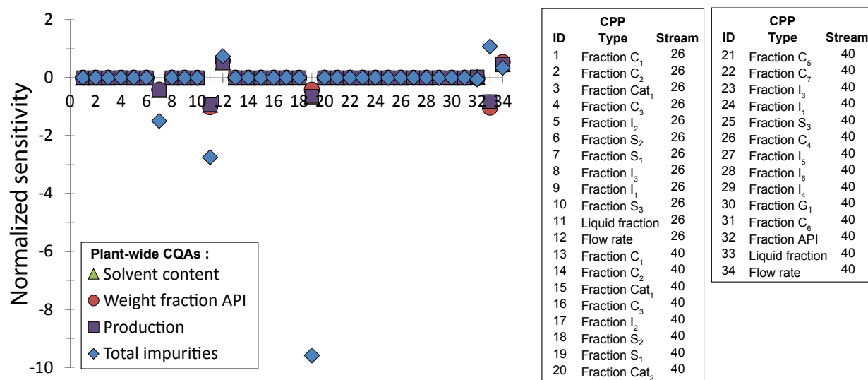
Figure 5: Steady-state values of the normalized sensitivities of the CQAs with respect to the CPPs at Level 2. The stream numbers that are used to explain the CPPs refer to 1. The fraction of the various compounds in the table with CPPs refers to the mass-based fraction of the liquid phase. The liquid fraction (CPP #11 and #33) is the volume-based liquid fraction of the slurry. The numerical values of the sensitivities are available as Supplementary Material.
