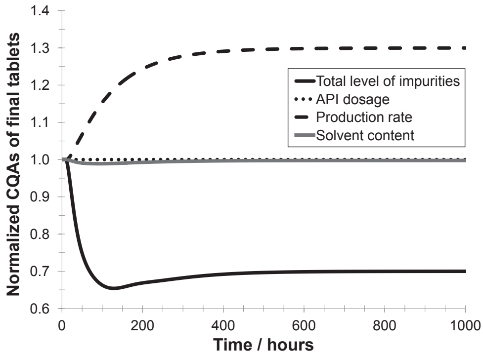
Figure 16: Dynamic development of four CQAs of the final product stream as a result of a step-change in the setpoints of the production rate and total level of impurities at t = 0 (+30% and -30% respectively). The solid black (bottom) line represents the dynamic development of the total level of impurities, the dotted black line (circles) represents the dynamic development of the API dosage, the gray line represents the dynamic development of the solvent content, and the dashed black line represents the dynamic development of the production rate.
