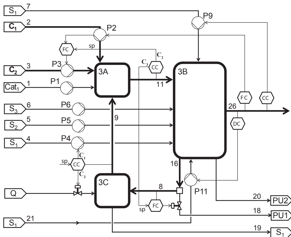
Figure 9: Representation of the continuous pharmaceutical pilot plant at Level 3 of the decomposition strategy. Block 2A from Level 2 (see 4) has been expanded to visualize the recycle structure. Block 3A contains all unit operations related to the first reaction, which produces the intermediate impurity I_1 . Block 3B represents all unit operations that are used to separate the reaction products into a stream that is rich in impurity I_1 (Stream 26) and a stream that is rich in reactant C_1 (Stream 16), which is partially purged (Stream 18) and send to a flash evaporator (Block 3C) to remove solvent S_1 (Stream 19) before the material returns to the reaction section (Stream 9). The control loops aim to control the CQAs of the streams that constitute the recycle to minimize the propagation of disturbances to the CQAs of Stream 26, which are critical at a higher level of the decomposition.
