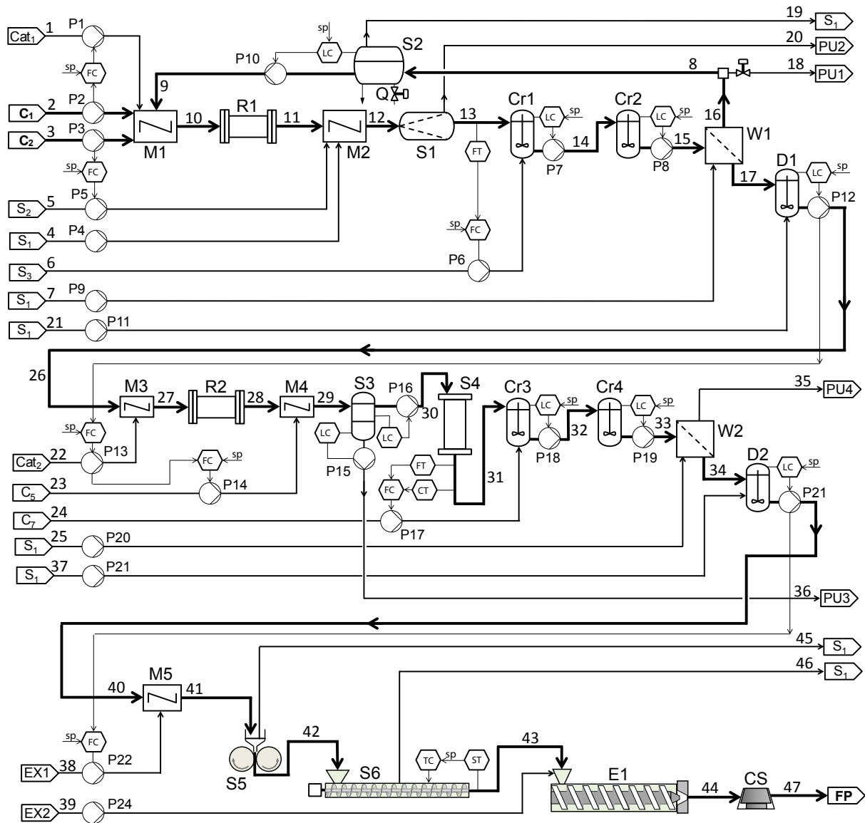
Figure 13: Representation of the continuous pharmaceutical pilot plant at the most detailed level of the decomposition strategy. The control structure contains all stabilizing control loops and the control loops that are synthesized at Level 4 of the decomposition to satisfy local control objectives.
