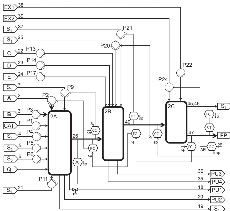
Figure 4: Representation of the continuous pharmaceutical pilot plant at Level 2 of the decomposition strategy. Block 2A entails all unit operations related to production of the first intermediate compound. Block 2B is dedicated to the synthesis and purification of the final API and Block 2C involves the formulation of the API. The control loops aim to control the properties of the intermediate streams that are critical to the quality of the final product.
