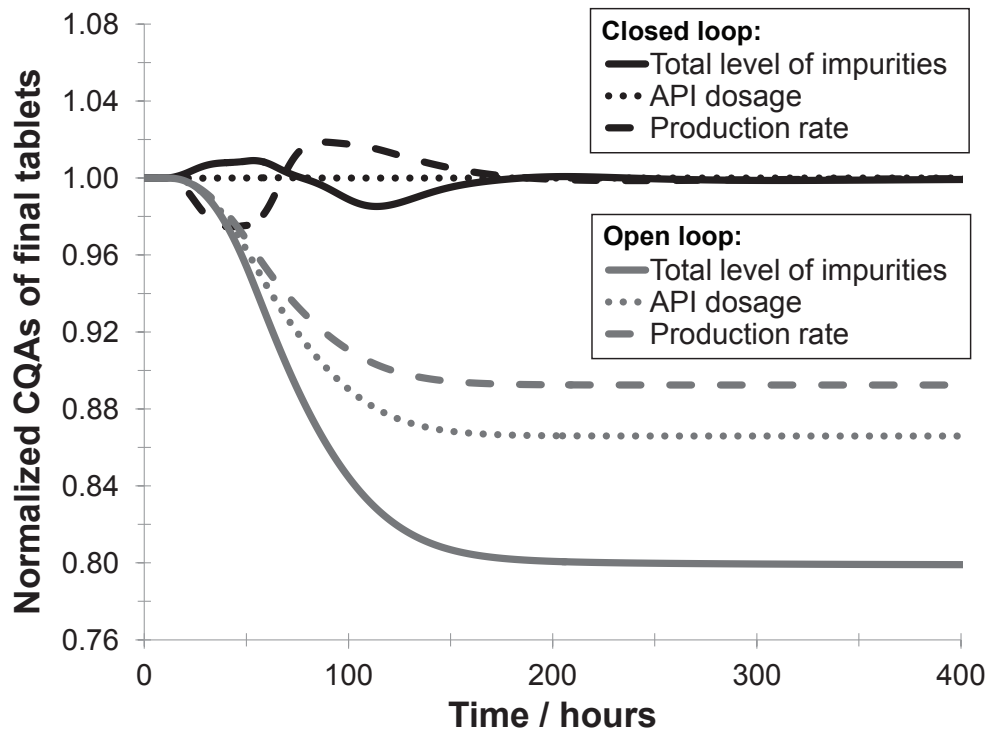
Figure 14: Dynamic development of three CQAs of the final product stream for a disturbance in the flow rate of fresh reactant C_1 (Case I). The black lines illustrate the closed-loop response and the gray lines illustrate the response with a stabilizing control layer only. The solid lines represent the dynamic development of the total level of impurities, the dotted lines represent the dynamic development of the API dosage, and the dashed lines represent the dynamic development of the production rate.
