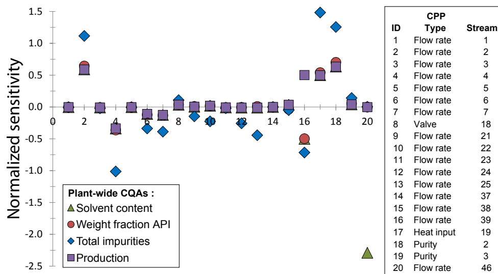
Figure 3: Steady-state values of the normalized sensitivities of the CQAs with respect to the CPPs at Level 1. The stream numbers that are used to explain the CPPs refer to 1. The numerical values of the sensitivities are available as Supplementary Material.
