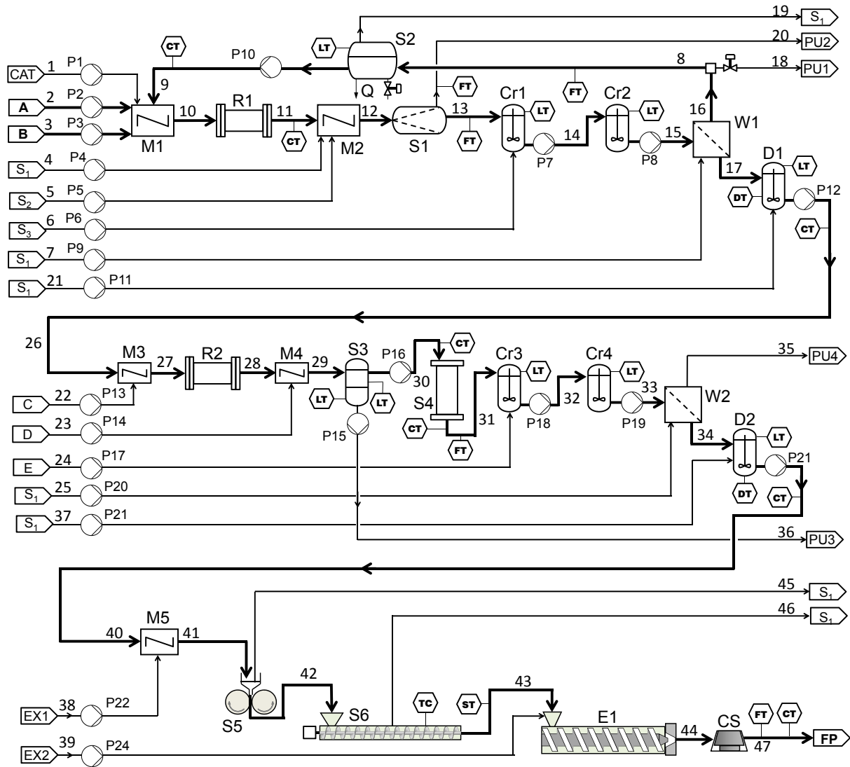
Figure 1: Process flowsheet
