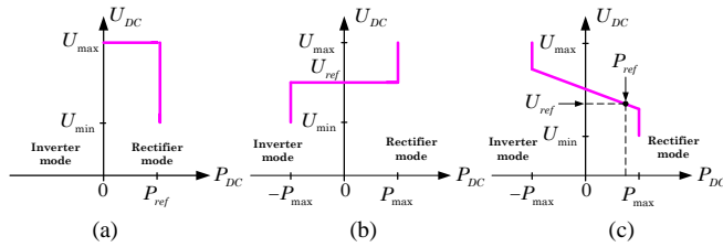
Figure 1. DC voltage versus power characteristics. (a). DC bus power controller (b). DC voltage regulator (c). DC voltage droop controller.
