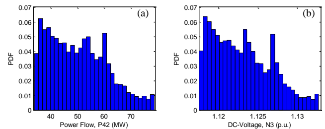
Fig. 1. Results of Scenario II.A3. Probabilistic density function: (a) power flow and (a) DC-voltage.
