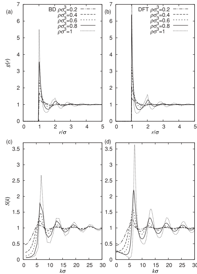
FIG. 1. (a) and (b) Display radial distribution functions, and (c) and (d) static structure factors for a bulk fluid of hard spheres at densities \rho\sigma^3 = 0.2, 0.4, 0.6, 0.8, and 1 . (a) and (c) are obtained from BD simulations and (b) and (d) via Percus' static test particle limit using the RY functional.
