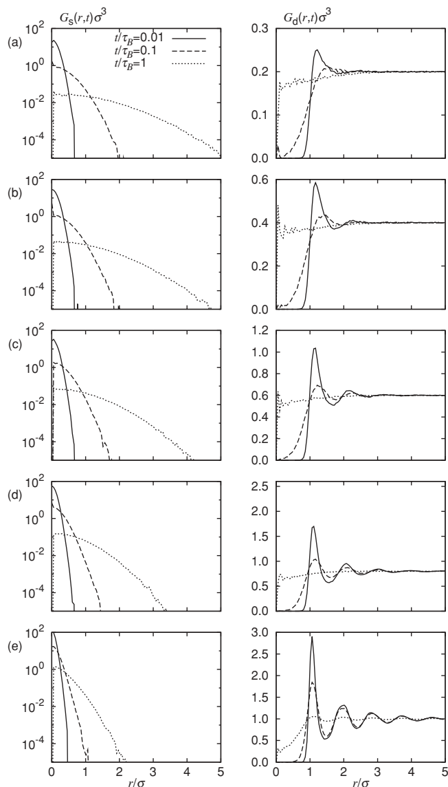
FIG. 2. The self and distinct parts of the van Hove distribution function, G_s(r, t) and G_d(r, t) , for a hard sphere fluid, measured in BD simulations at densities: (a) \rho\sigma^3 = 0.2 , (b) \rho\sigma^3 = 0.4 , (c) \rho\sigma^3 = 0.6 , (d) \rho\sigma^3 = 0.8 , (e) \rho\sigma^3 = 1 . The results are plotted for times t/\tau_B = 0.01 (solid line), 0.1 (dashed line), and 1 (dotted line). In the semi logarithmic scale of G_s(r, t) versus r a Gaussian appears as a parabola. The G_d(r, t) results are shown on a linear scale.
