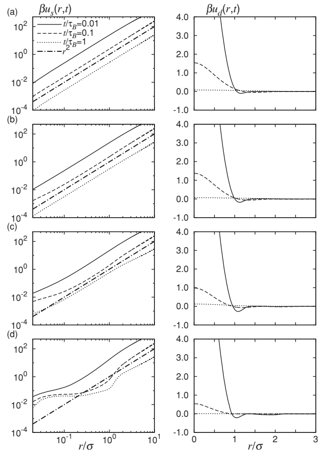
FIG. 9. External potentials, u_s(r, t) and u_d(r, t) , required to generate equilibrium density profiles, \rho_s(r, t) and \rho_d(r, t) , identical to those obtained from the dynamical test particle approach—see Fig. 3. The external potentials also include an overall time-dependent additive constant which is not indicated. Note the logarithmic x -axis for u_s(r, t) . At low densities u_s(r, t) is approximately parabolic, as indicated by the straight line (dashed-dotted). At high densities u_s(r, t) is distorted at small r , but still parabolic at large r .
