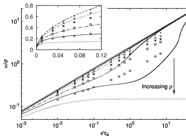
FIG. 5. The width w of the self part of the van Hove function, defined in Eq. (11), measured in the BD simulations for \rho\sigma^3 = 0.2 (+), 0.4 (x), 0.6 (*), 0.8 (□), and 1 (○), and from the dynamical test particle theory, for \rho\sigma^3 = 0.2 (long dashed line), 0.4 (short dashed line), 0.6 (dashed-dotted line), 0.7 (solid line), and 0.8 (dotted line). Also shown is the result from the Vineyard approximation (thick solid grey line). In the main panel both axes are logarithmic; the inset displays the same results on linear scales.
