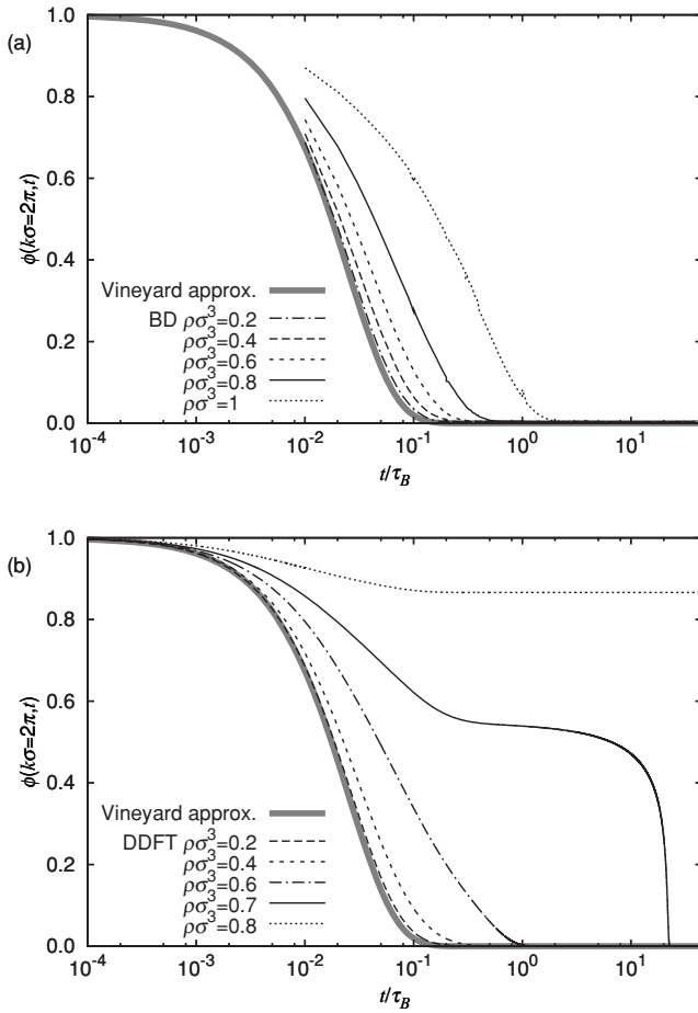
FIG. 8. Scaled intermediate scattering function \phi(k\sigma = 2\pi t) as a function of time t/\tau_B , calculated from the Vineyard approximation (thick gray line) compared to (a) BD simulation results and (b) the dynamical test particle method. The dynamical test particle results exhibit slowing and arrested dynamics for \rho\sigma^3 = 0.7 and 0.8 .
