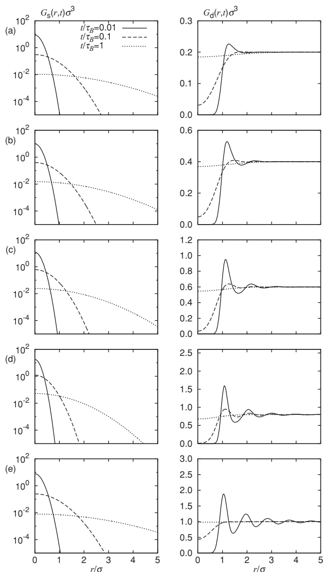
FIG. 4. The self and distinct parts of the van Hove distribution function, G_s(r, t) and G_d(r, t) , calculated using the Vineyard approximation for densities: (a) \rho\sigma^3 = 0.2 , (b) \rho\sigma^3 = 0.4 , (c) \rho\sigma^3 = 0.6 , (d) \rho\sigma^3 = 0.8 , (e) \rho\sigma^3 = 1 . The results are plotted for times t/\tau_B = 0.01 (solid line), 0.1 (dashed line), and 1 (dotted line).
