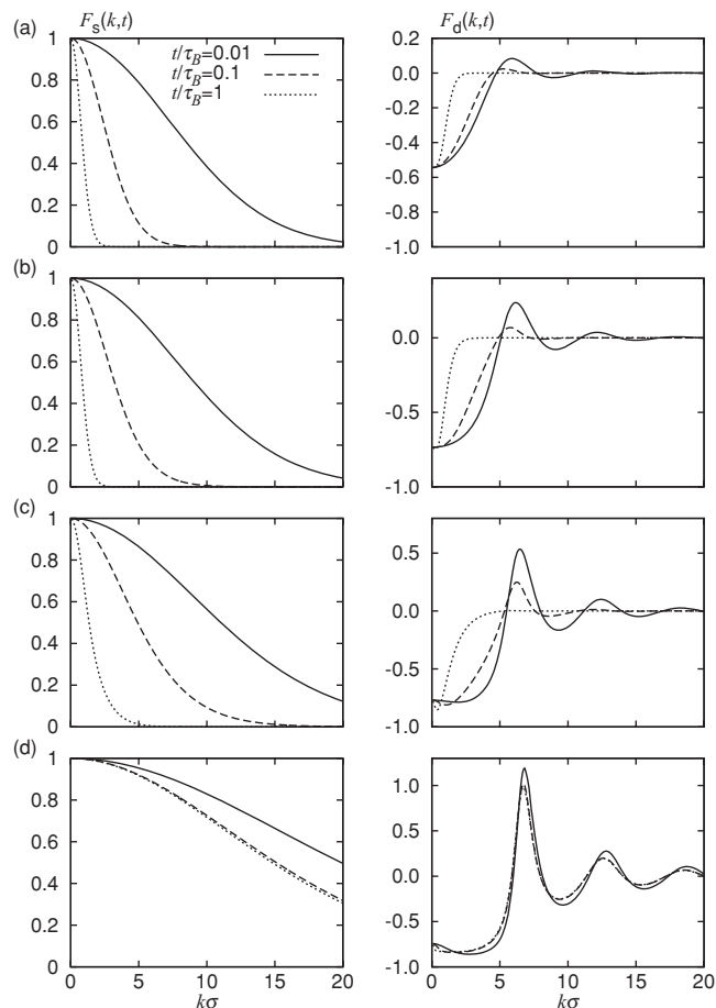
FIG. 7. Intermediate scattering functions F(k, t) , obtained by a spatial Fourier transform, Eq. (12), of the dynamic test particle density profiles, \rho_s(r, t) and \rho_d(r, t) , displayed in Fig. 3.
