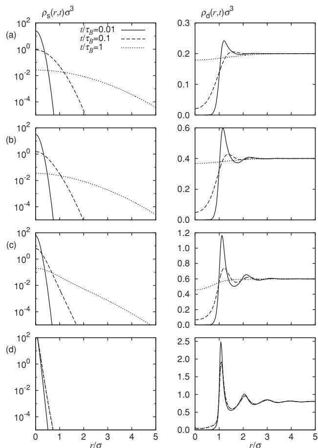
FIG. 3. The “s” and “d” density profiles, \rho_s(r, t) and \rho_d(r, t) , obtained from the dynamical test particle theory, for densities: (a) \rho\sigma^3 = 0.2 , (b) \rho\sigma^3 = 0.4 , (c) \rho\sigma^3 = 0.6 , (d) \rho\sigma^3 = 0.8 . The results are plotted for times t/\tau_B = 0.01 (solid line), 0.1 (dashed line), and 1 (dotted line). In (d), after a short time, the system reaches an “arrested state,” where the density profiles no longer evolve in time and the width of \rho_s(r, t \rightarrow \infty) remains finite.
