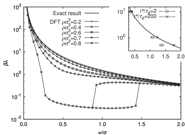
FIG. 13. The (scaled) strength of the parabolic potential, \beta\lambda , versus the resulting width, w/\sigma , of \rho_s(r) . Results are calculated using the equilibrium DFT and compared to the exact result. For the bulk fluid densities \rho\sigma^3 = 0.2, 0.4, 0.6 , and 0.7 , \lambda decreases monotonically with w . However, for \rho\sigma^3 = 0.8 the curve is no longer monotonic, and exhibits two disconnected branches. The inset shows the effect of insufficient simulation run times on the equivalent situation studied using BD computer simulations, where t^* is the simulation run time.
