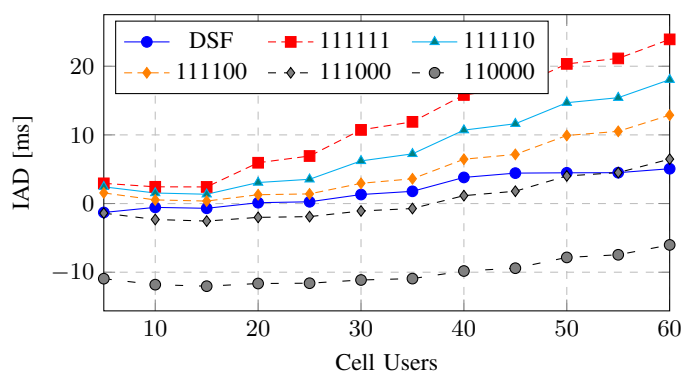
Fig. 9. Results for Inter Arrival Difference with increasing cell users; illustrating the time difference in arrival of the joint unicast and broadcast streams to a given HUBS subscriber with DSF or Static SF map allocation.
