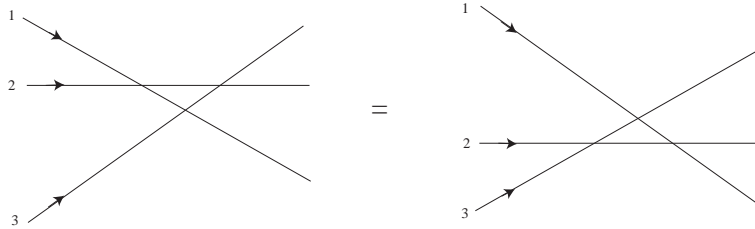
Figure 1: Yang-Baxter relation
