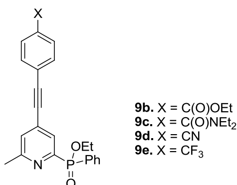
Scheme 3. Structure of the phenylphosphinate model chromophores 9b-e featuring electron withdrawing substituents.
