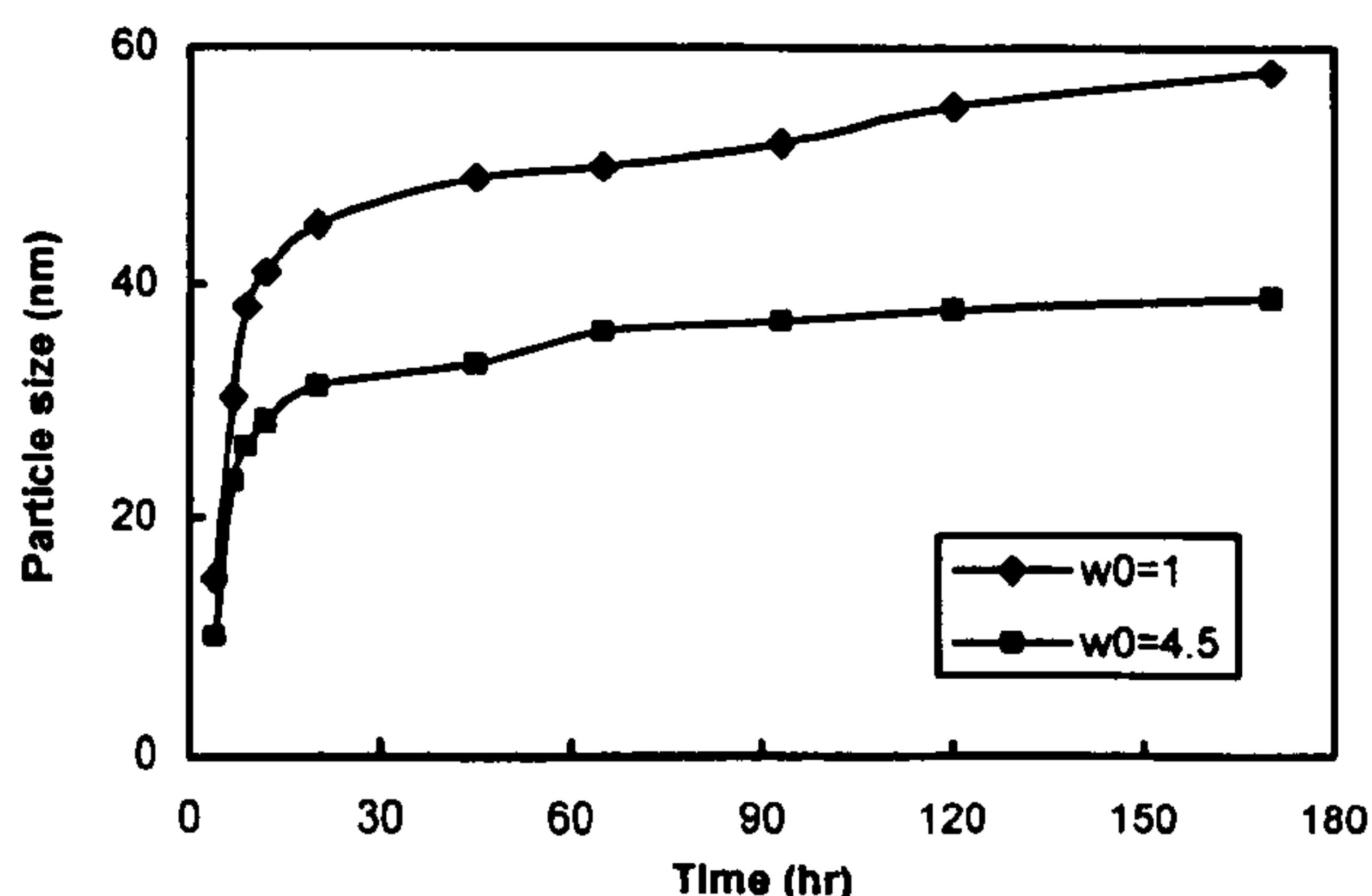
Figure 2.5-23 Silica particle growth kinetics measured by DLS at different values of \omega_0 = [\text{H}_2\text{O}] / [\text{Surfactant Tx-45}] [62] .
