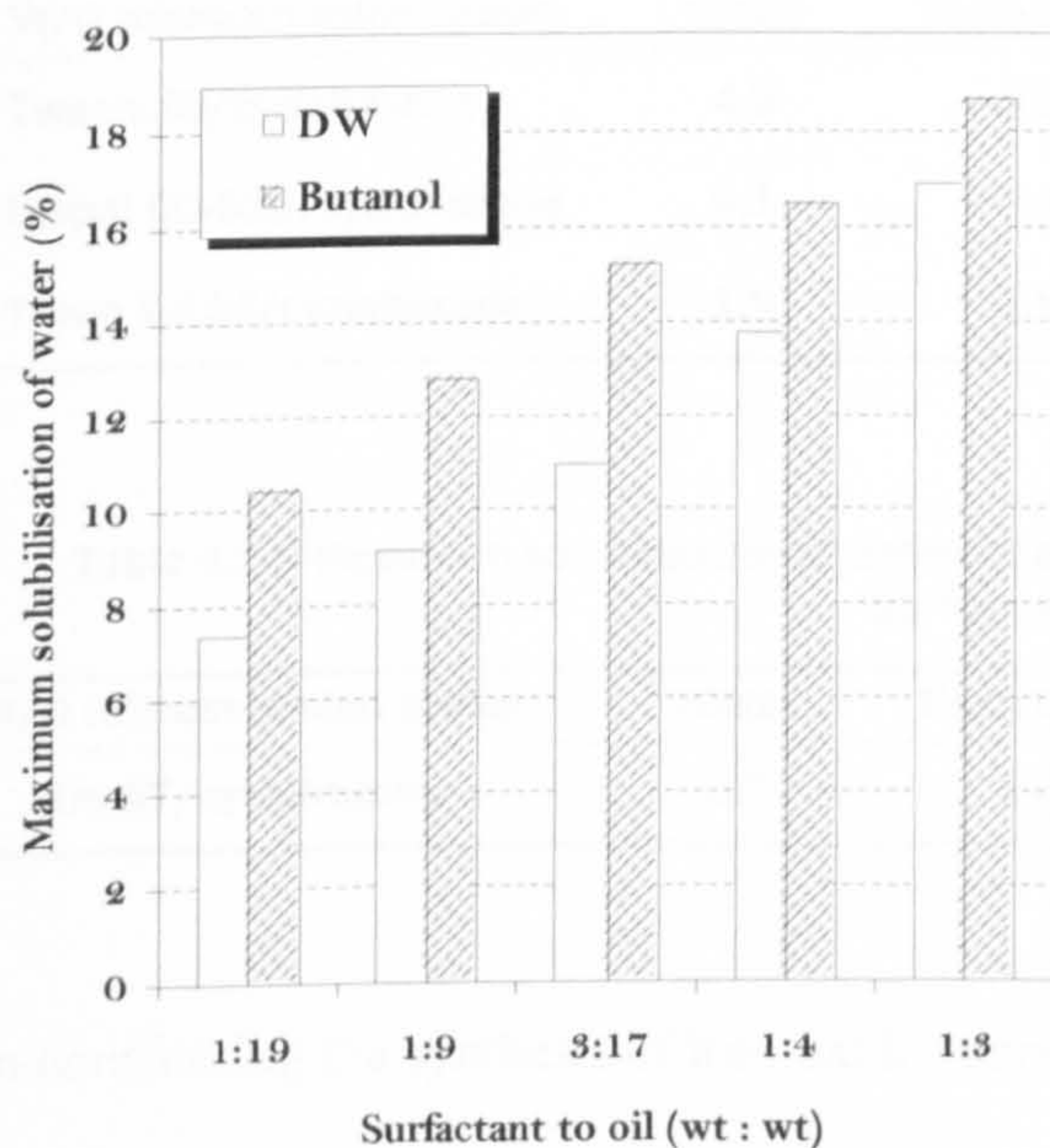
Figure 4.1-7 Maximum solubilisation of water in Igepal CO-520/cyclohexane system with butanol applied as co-surfactant at 25°C.
