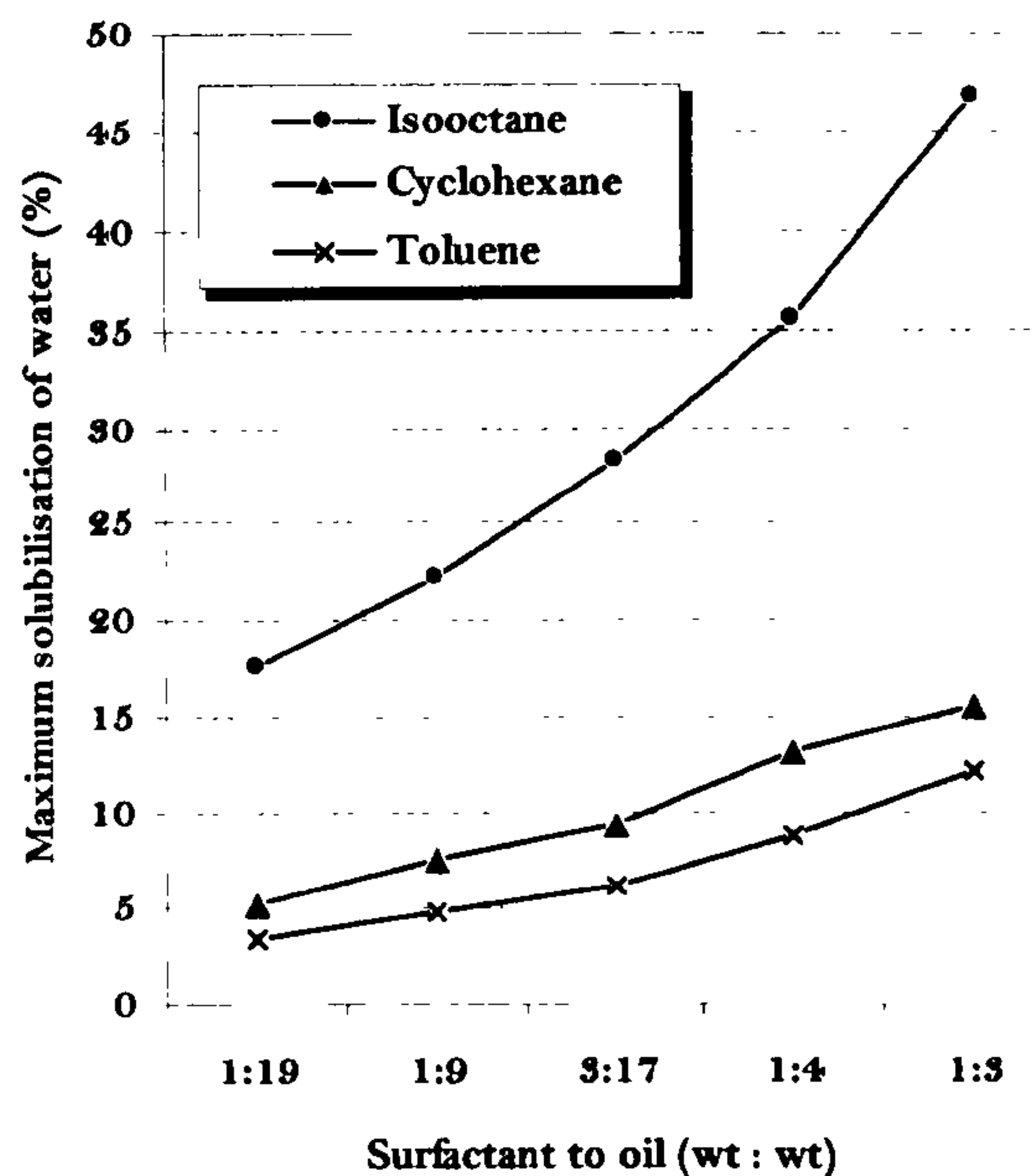
Figure 4.1-4 Maximum solubilisation of water in AOT systems at 25°C.
