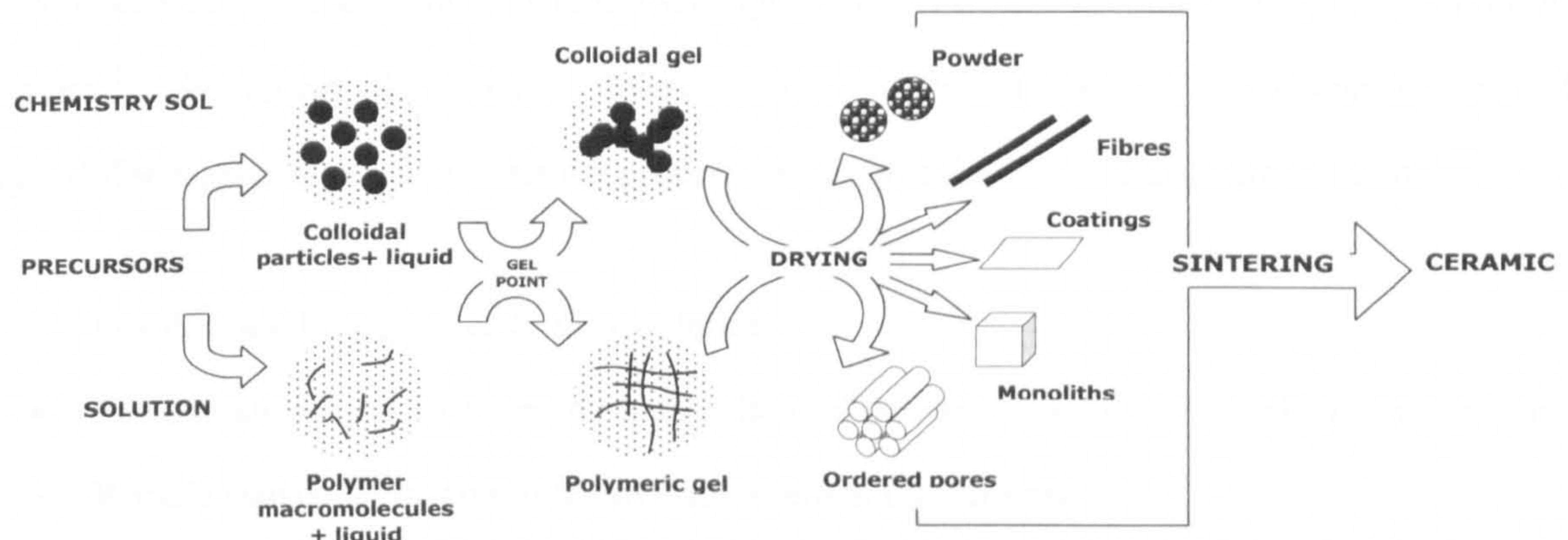
Figure 2.2-3 Schematics of sol-gel process.
