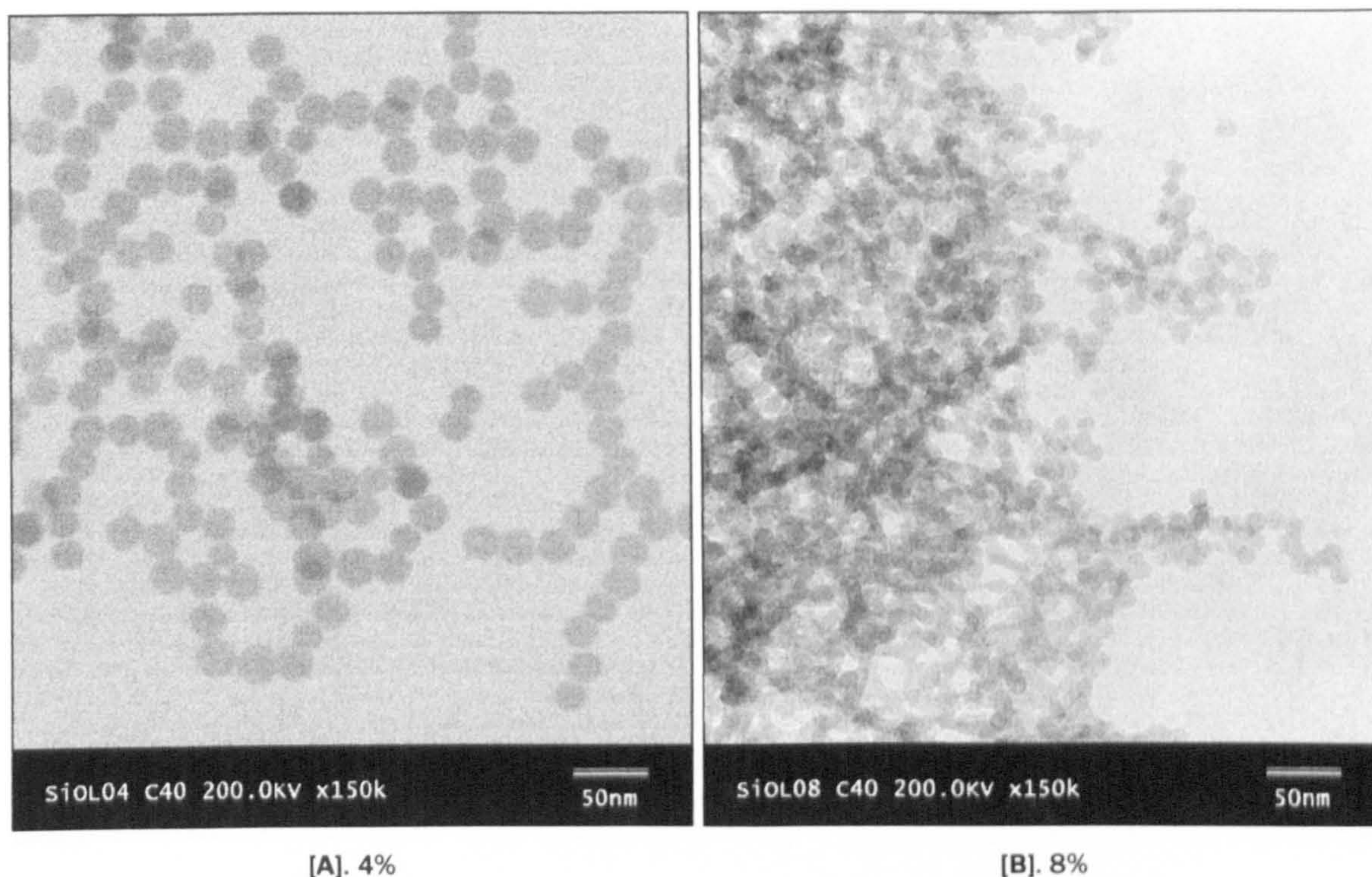
Figure 7.1-3 TEM micrographs of silica nano-spheres prepared via Igepal CO-520/cyclohexane w/o microemulsion with different loadings of aqueous phase at 25°C for 24 hours. Surfactant : oil = 1:4 (wt:wt).
