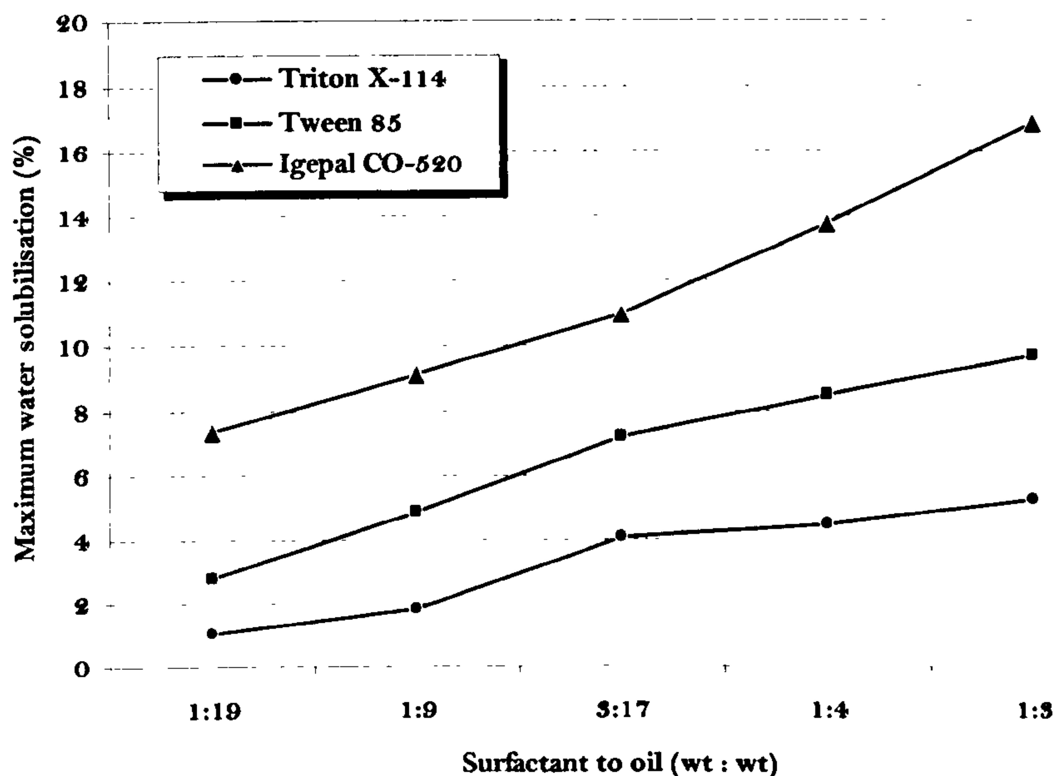
Figure 4.2-2 Effect of different surfactants on the maximum water solubilisation in w/o microemulsion systems with cyclohexane as the oil phase at 25°C.
