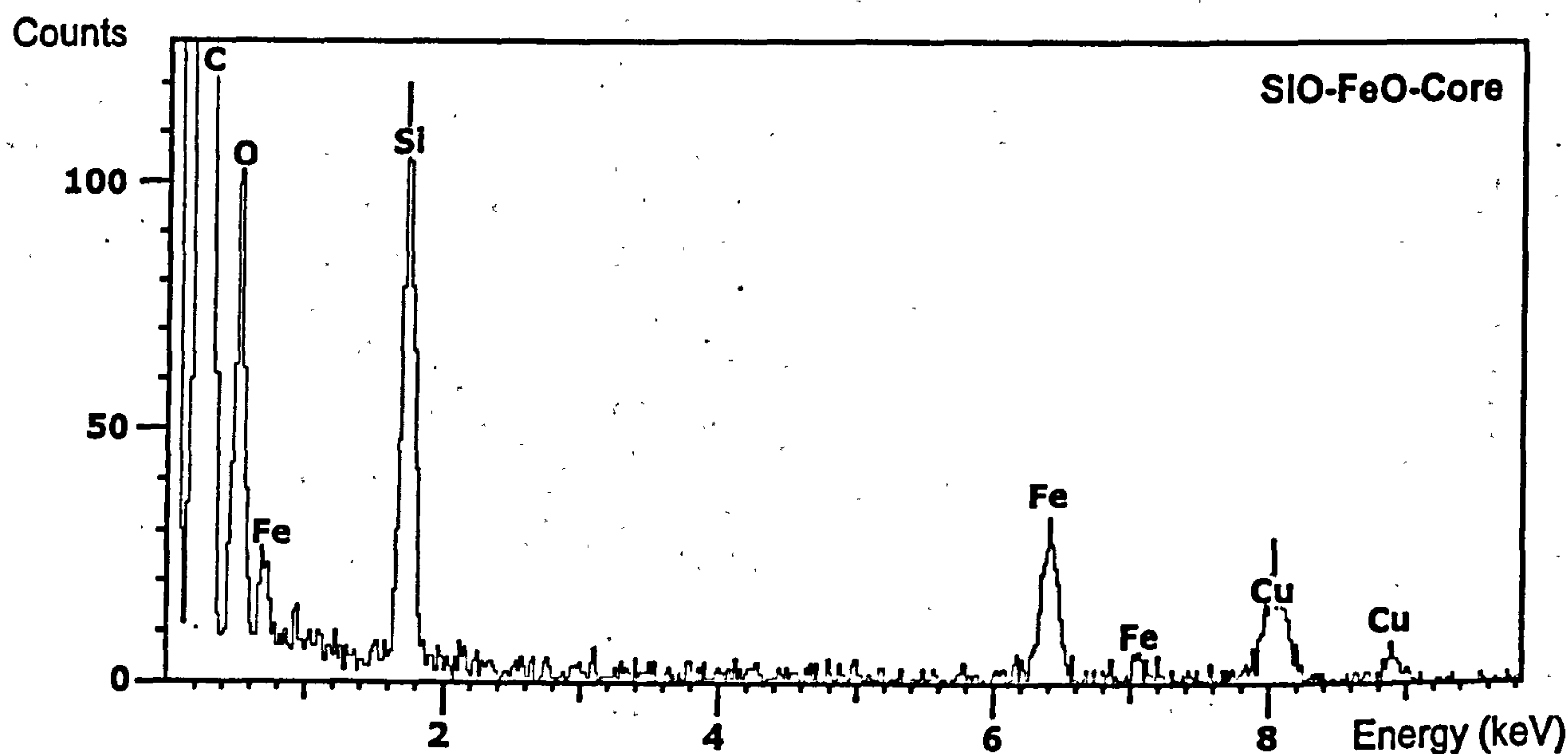
Fig.7.EDX analysis of (top) outer layer and (bottom) central part of the nanoparticle.
