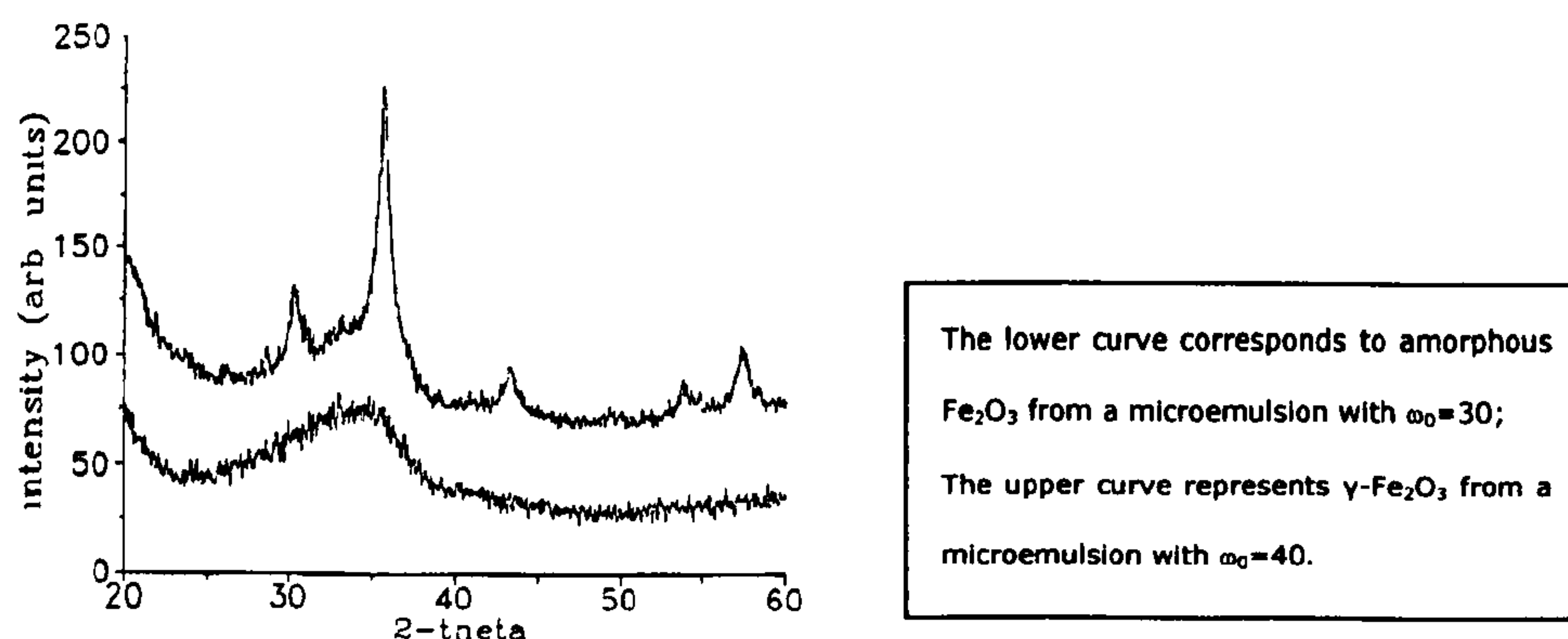
Figure 2.5-6 XRD of the Fe 2 O 3 particles produced via the microemulsion followed by calcination at 225°C [139] .
