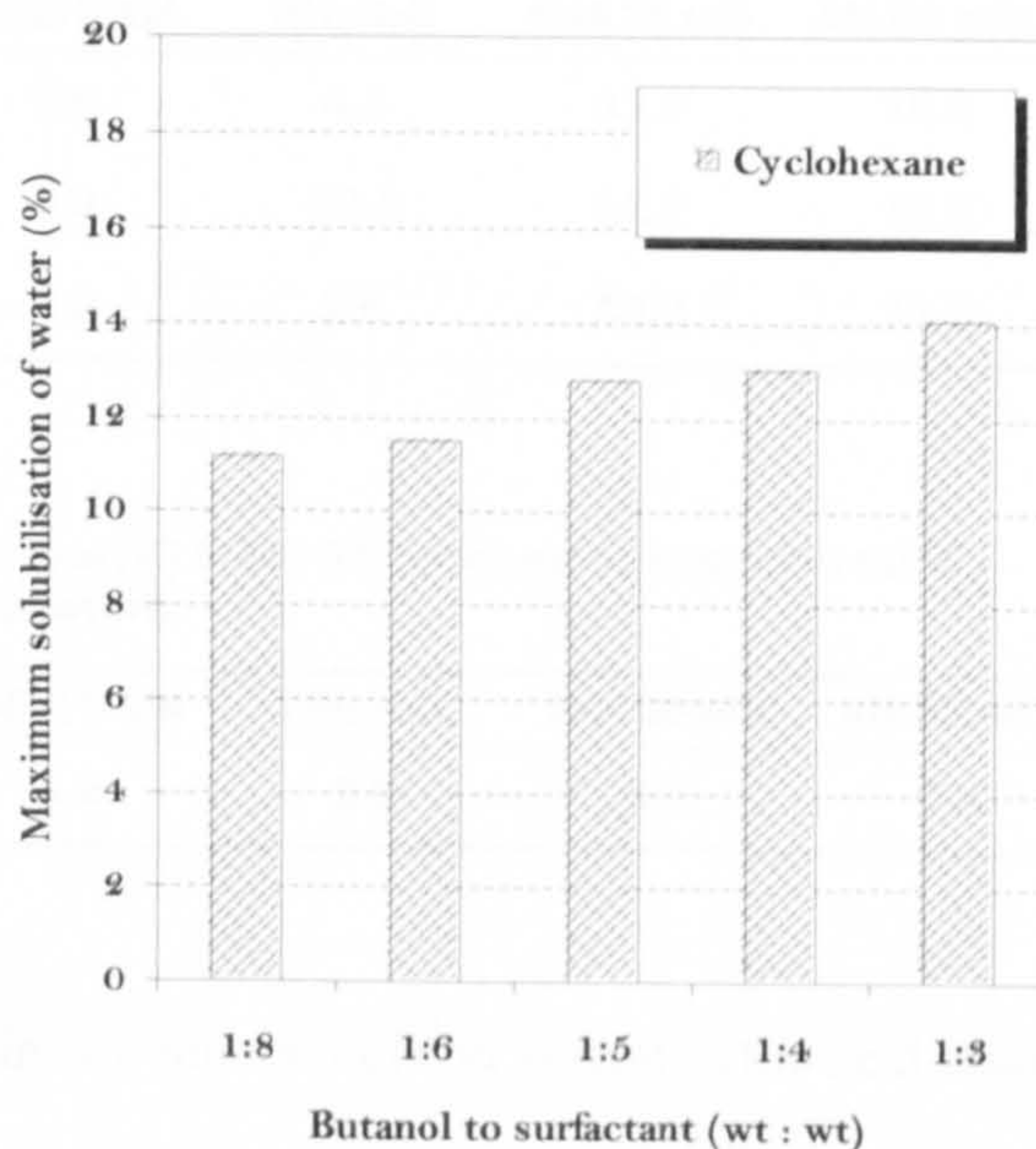
Figure 4.1-8 Maximum solubilisation of water in Igepal CO-520/butanol/cyclohexane system at 25°C.
