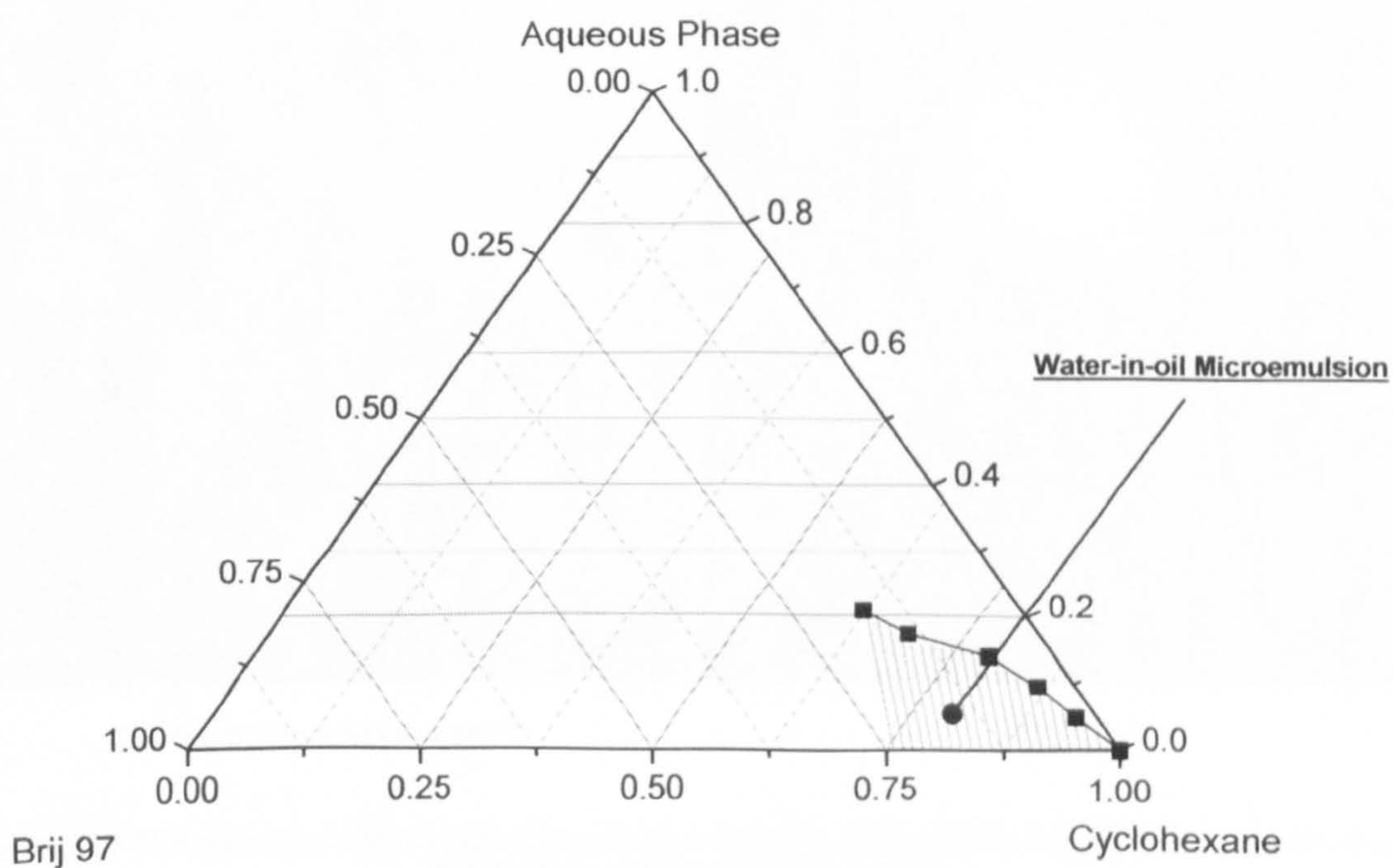
Figure 5.1-8 Phase diagram of w/o microemulsion system: Brij 97/cyclohexane/aqueous phase at 60°C.
