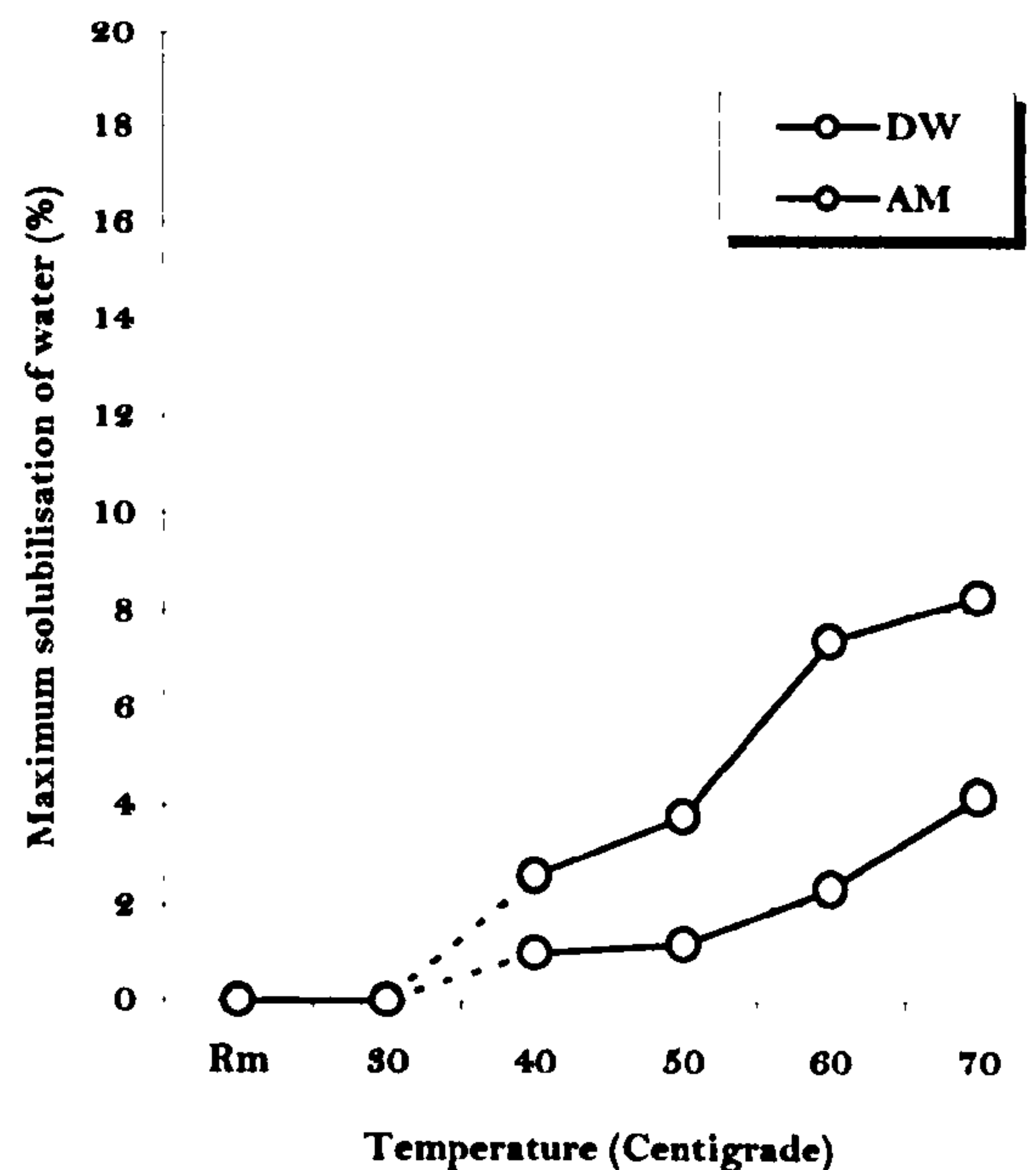
Figure 4.1-14 Maximum solubilisation of water in Brij 97/Cyclohexane system at different temperatures.
