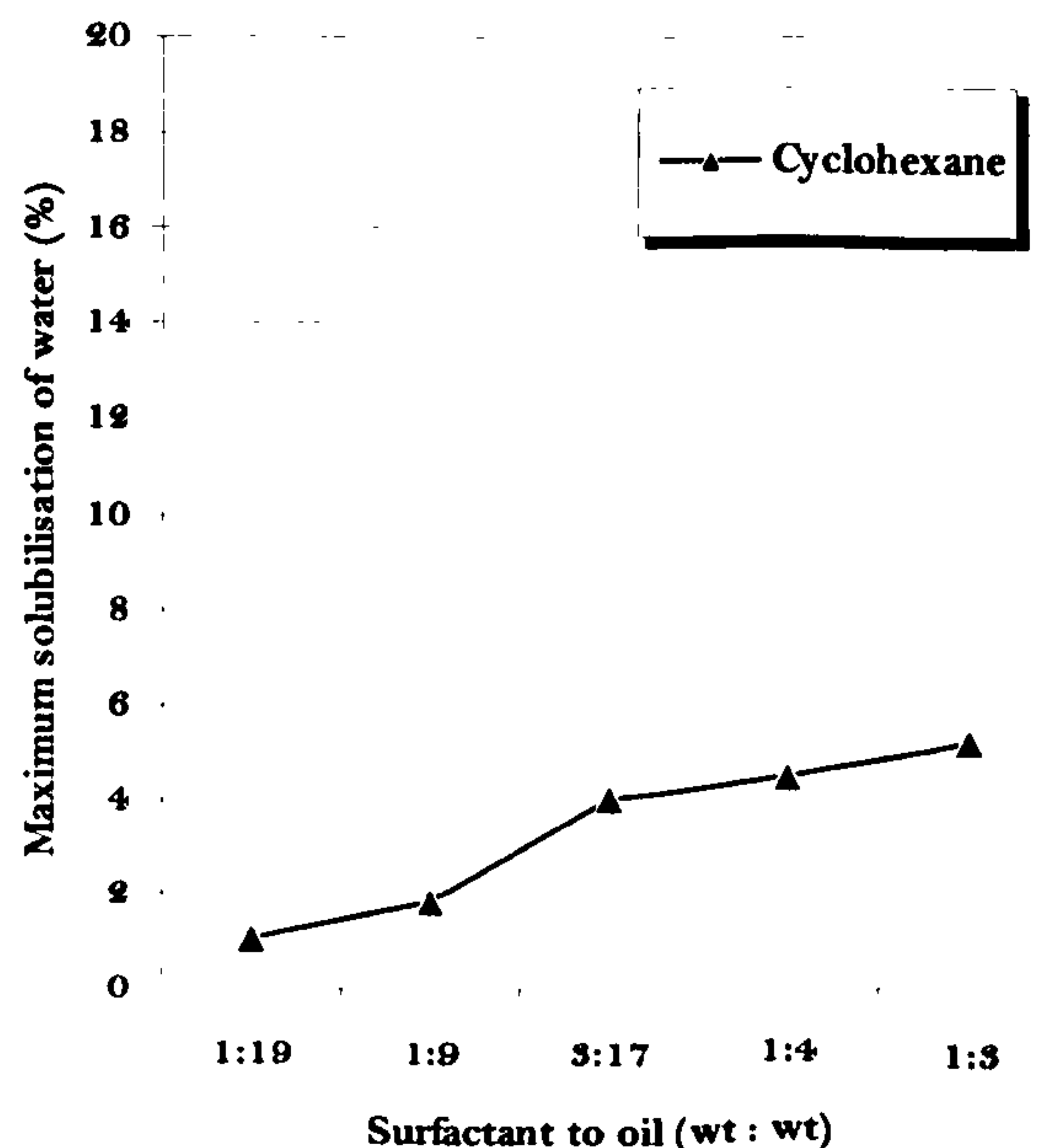
Figure 4.1-3 Maximum solubilisation of water in Triton X-114/cyclohexane system at 25°C.
