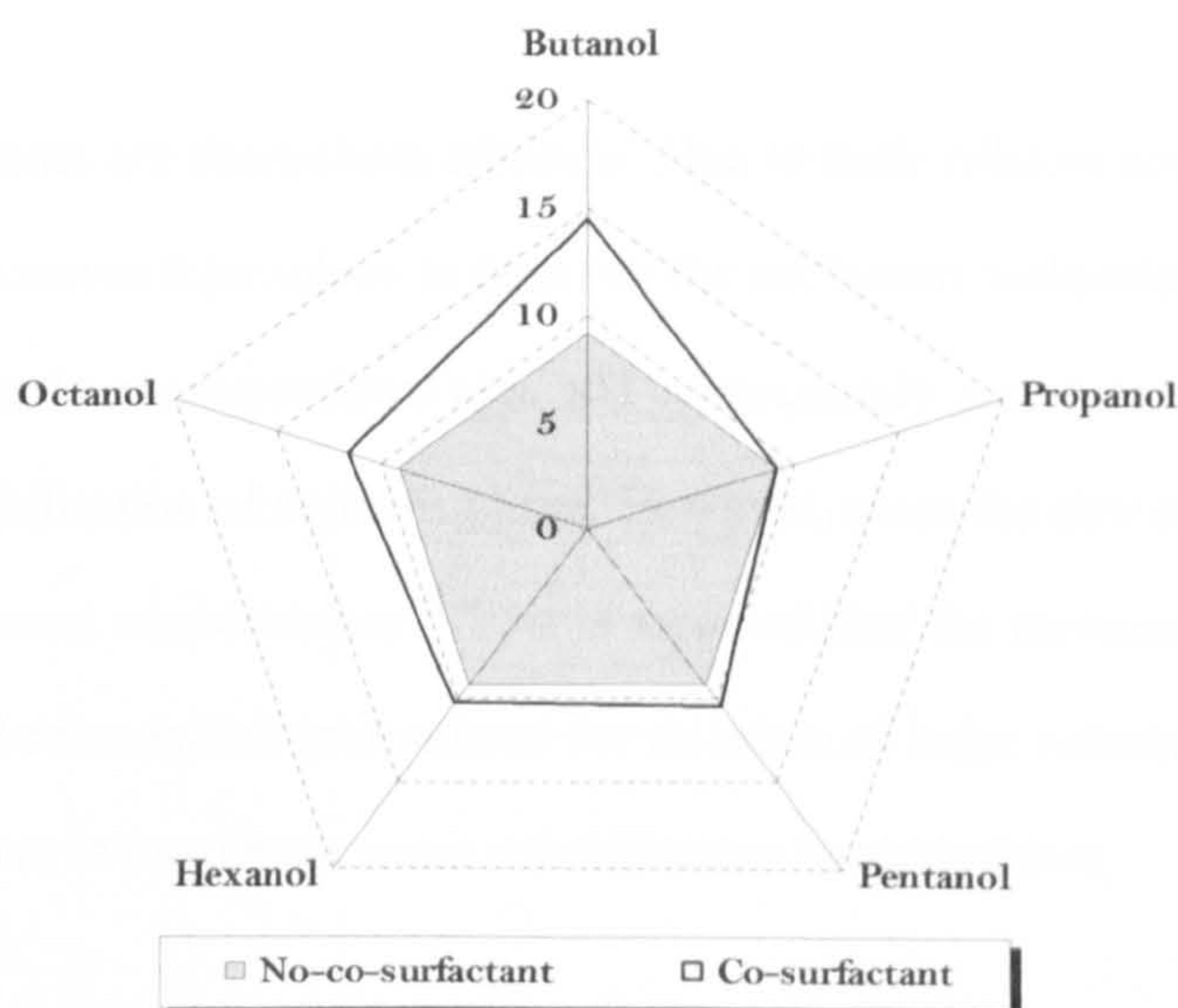
Figure 4.2-5 Maximum water solubilisation in Igepal CO-520/cyclohexane system with different co-surfactants applied at 25°C. Surfactant mixture: oil = 1:9 (wt:wt). Co-surfactant: Igepal CO-520 = 1:5 (wt:wt).
