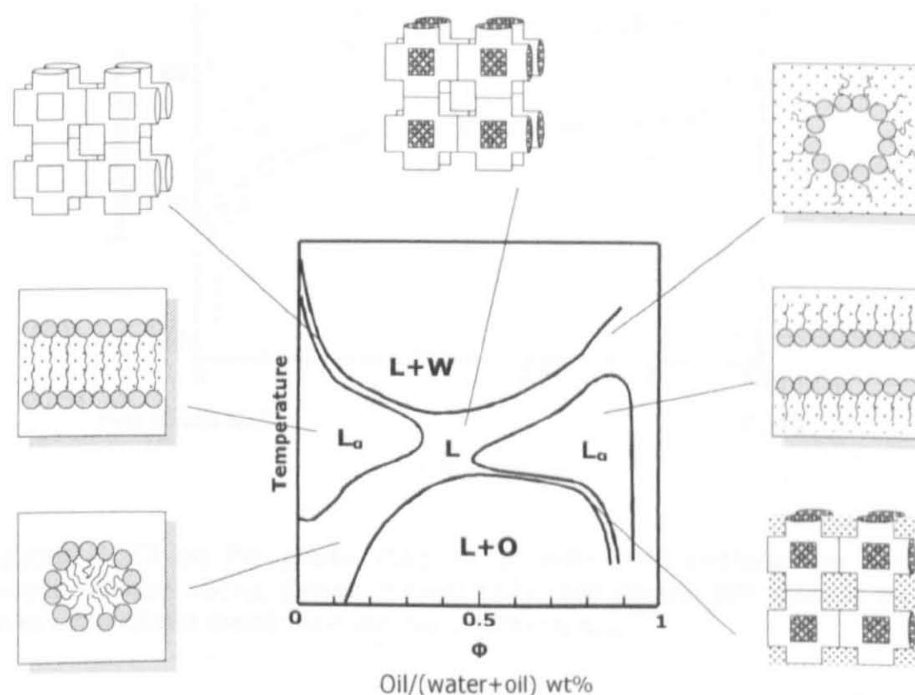
Figure 2.4-6 A schematic phase diagram and various micro-structures found in different regions of the liquid phase (microemulsion), L. At higher temperatures the liquid phase is in equilibrium with excess water (L+W), and at lower temperatures with excess oil (L+O) [85] .
