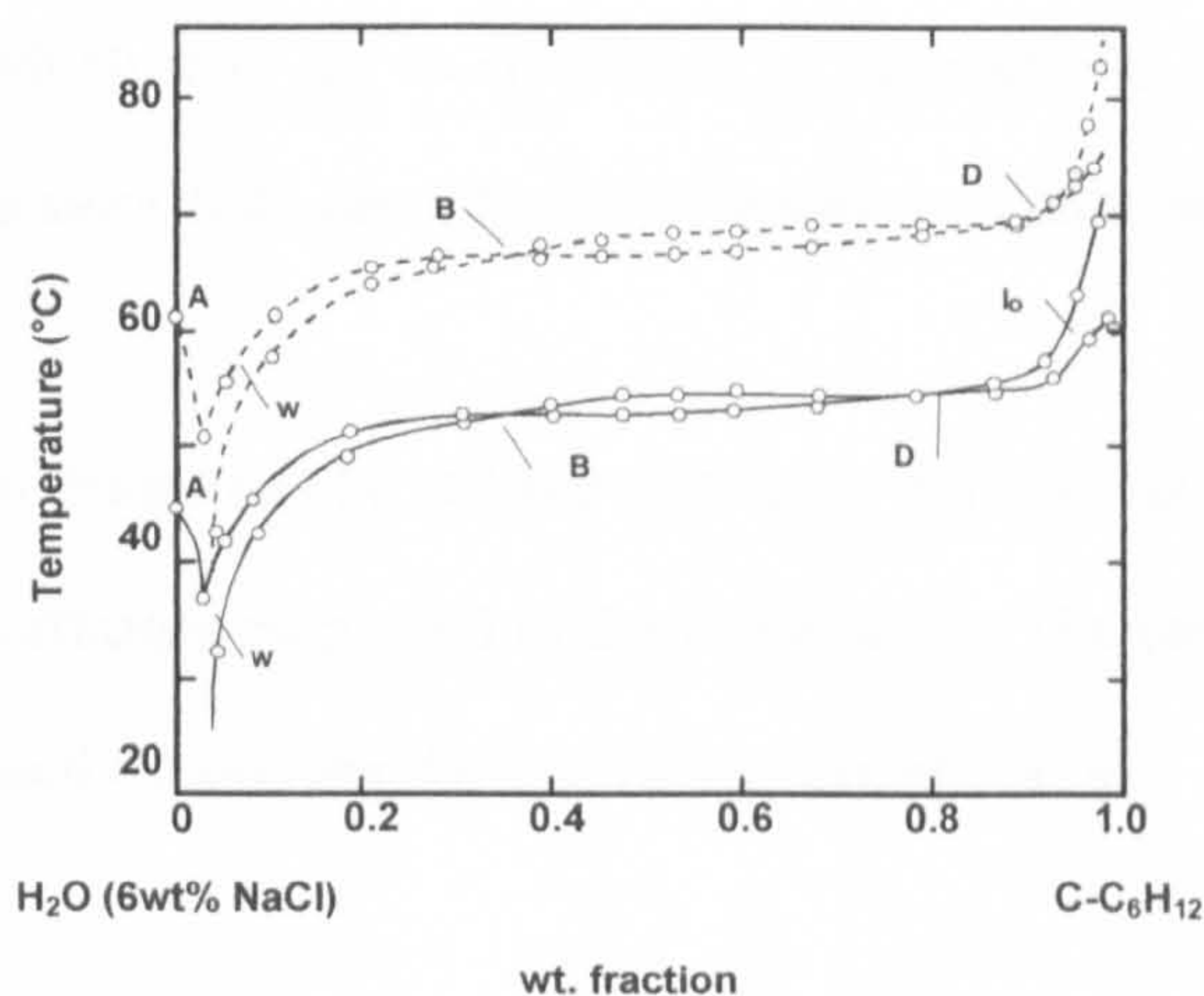
Figure 2.4-7 Effect of added NaCl on the phase diagram of water and cyclohexane containing 5 wt% \text{C}_9\text{H}_{19}\text{C}_6\text{H}_4\text{O}-(\text{CH}_2\text{CH}_2\text{O})_{9.7}\text{H} . Dotted curves: no salt added. Drawn curves: 6wt% salt added. Not that the equilibrium compositions of the phases occurring in two- and three-phase areas may change on adding salt [87] .
