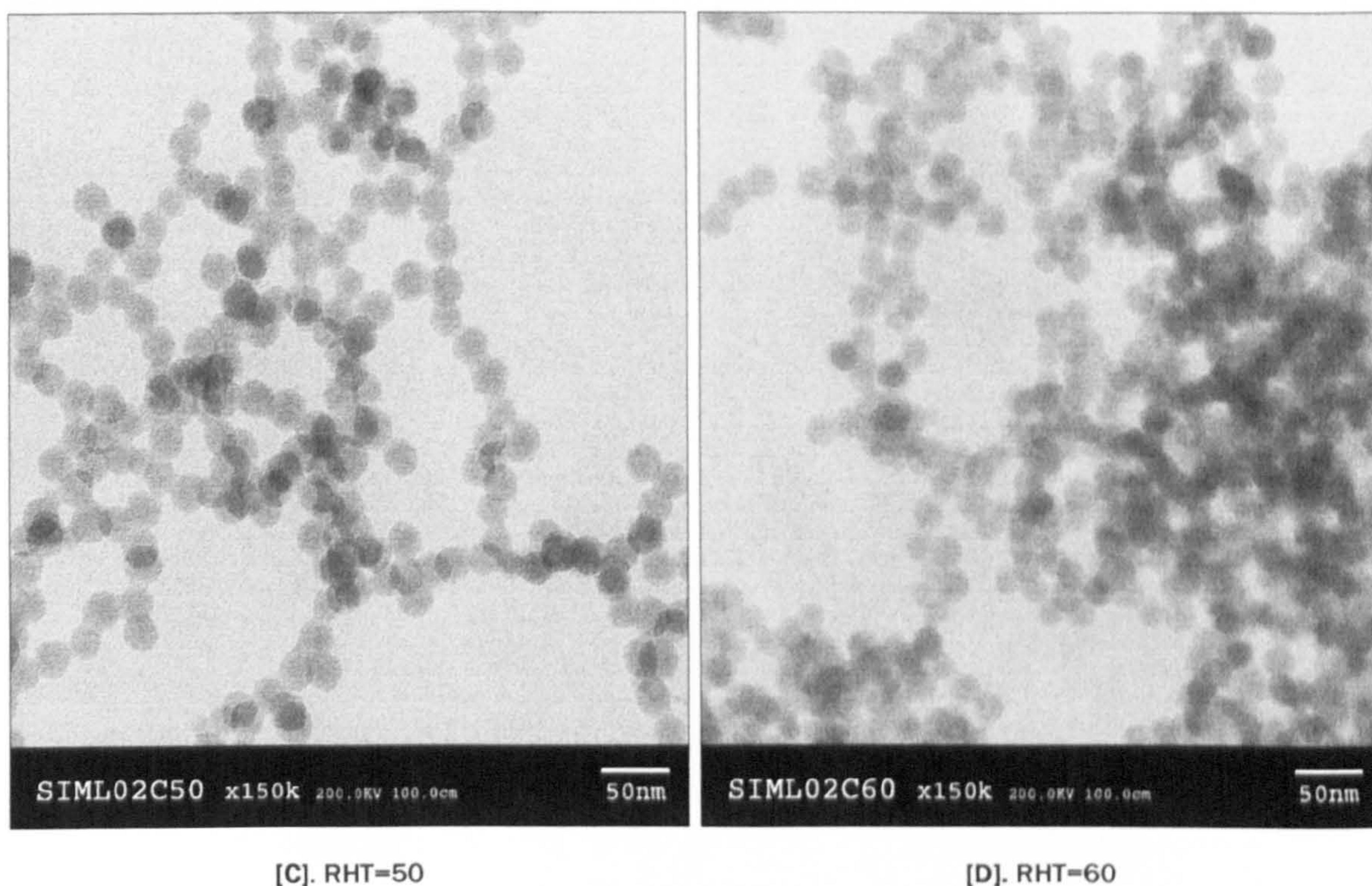
Figure 7.1-2 TEM micrographs of silica nano-spheres prepared via Igepal CO-520/cyclohexane w/o microemulsion at 25°C for 24 hours with the different molar ratios (RHT) of water to TEOS. Surfactant : oil = 1:4 (wt:wt)
