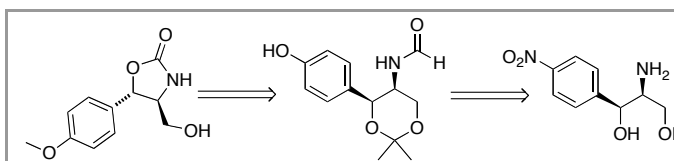
Scheme 1 Retrosynthetic route towards (4 S ,5 S )- iso -isocytoxazone
