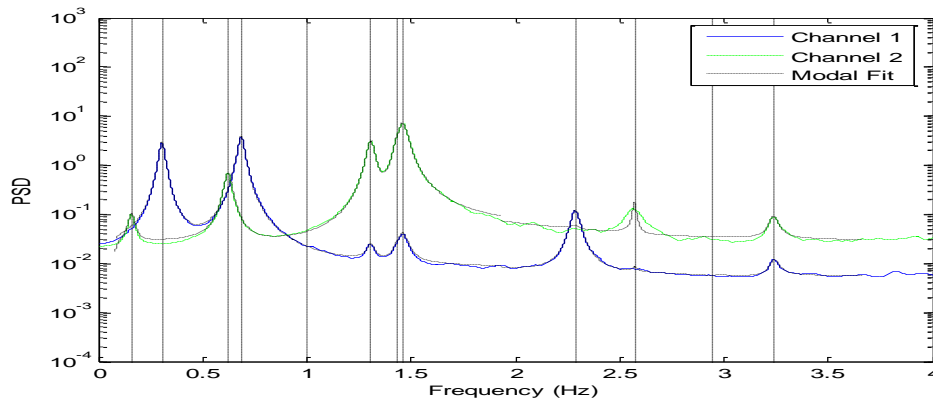
Figure 5. Comparison between measured and modal model predicted CPD.
