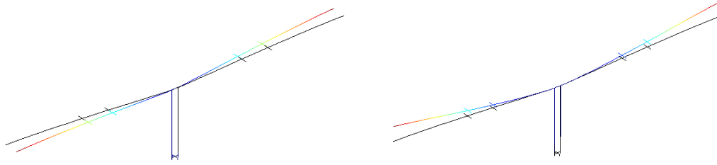
Figure 7: Modeshapes predicted by the finite element model of Metsovo bridge (a) 1 st (rotational) ( \omega = 0.1461 Hz), ( \beta ) 5 th (bending of the cantilevered deck \omega = 0.7257 Hz).
