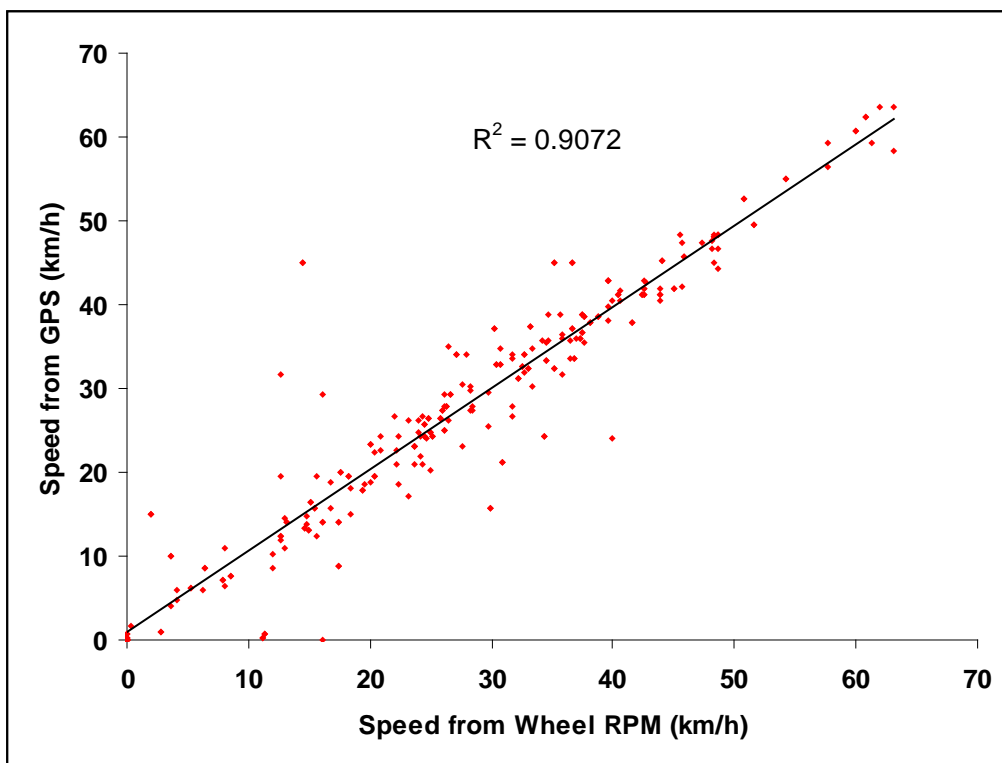
Figure 3: Correlation coefficient between GPS speed and wheel sensor measurements
