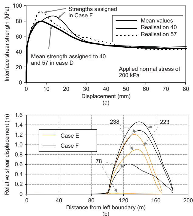
Figure 11. (a) Example variability of selected interface shear strengths in case F compared with mean strength used in realisations 40 and 57, case D; (b) comparison of relative shear displacement distributions for TGM-FINES interface computed in realisations 78, 223 and 238, cases E and F
