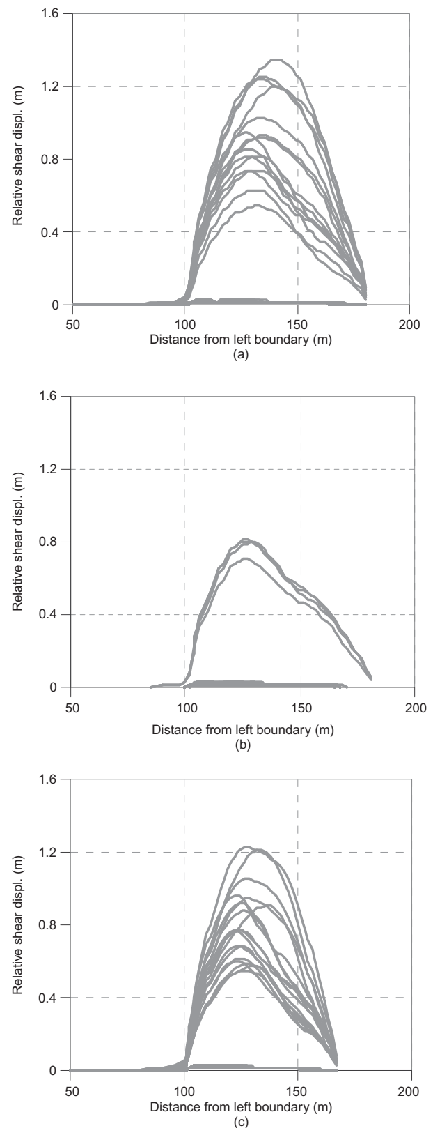
Figure 9. Relative shear displacement distributions along TGM-FINES interface after construction stage 6 for 1:2.0 slope: (a) case C; (b) case D; (c) case E
