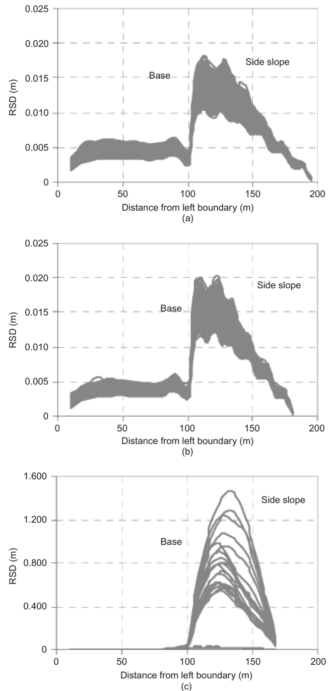
Figure 13. Relative shear displacement distributions along TGM-FINES interface after construction stage 6: (a) case G, 1:3.0 slope; (b) case A, 1:2.5 slope; (c) case F, 1:2.0 slope
