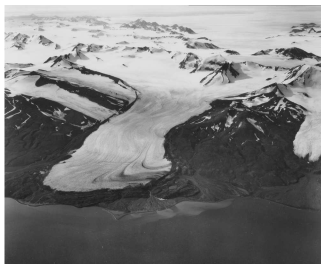
Fig. 3. Oblique aerial photograph of Finsterwalderbreen taken in 1936, looking southwards (© Norsk Polarinstitutt, photograph S36 3201). Note the looped moraines visible near the terminus and the displaced flowlines higher up the glacier.
