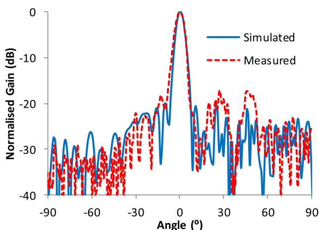
Fig. 8 Measured and simulated gain pattern at 30 GHz in the E-plane
