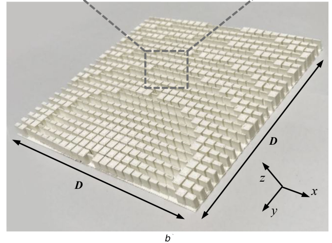
Fig. 2 Geometry of the 3D printed dielectric resonator reflectarray
