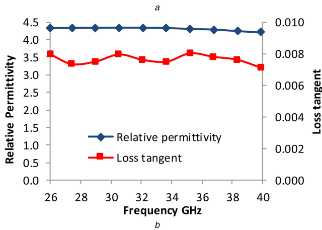
Fig. 1 Measurement of composite ABS material
